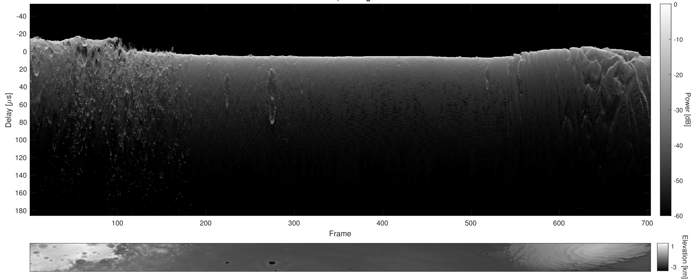
Orbit 22406, Cluttergram
