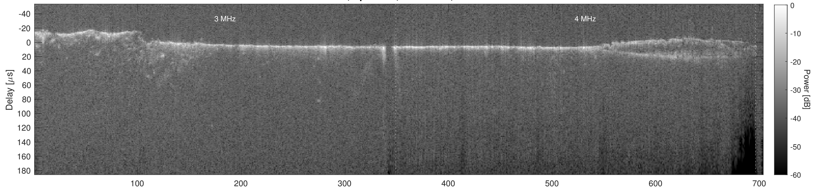
Orbit 22406, Cluttergram
