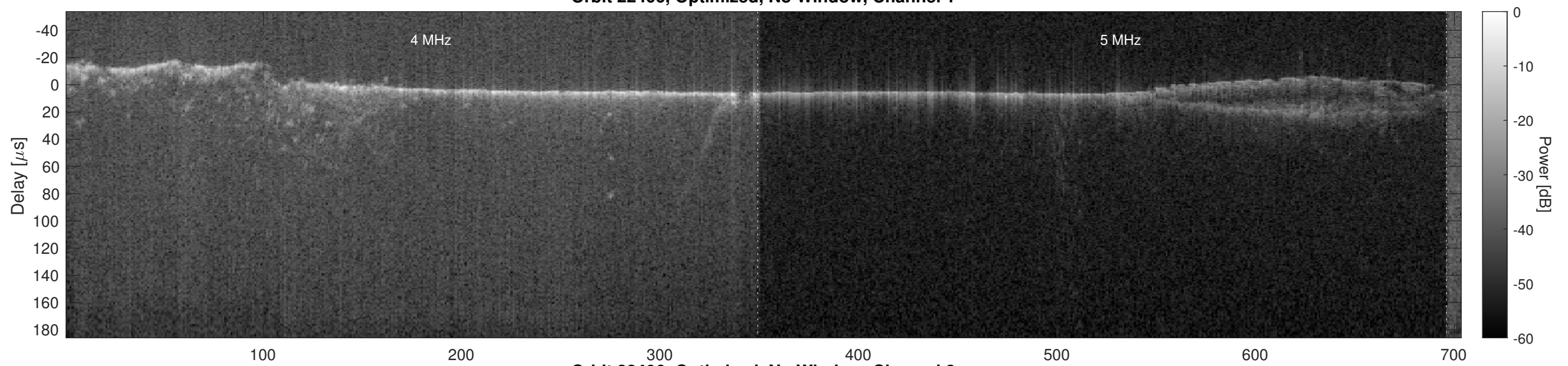
Orbit 22406, Optimized, No Window, Channel 2
