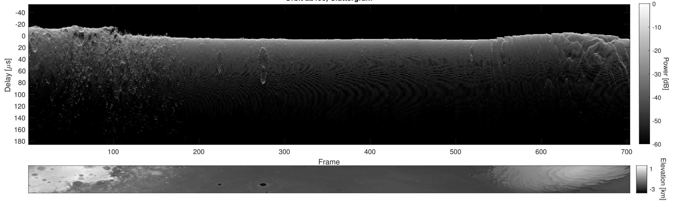
Orbit 22406, Cluttergram
