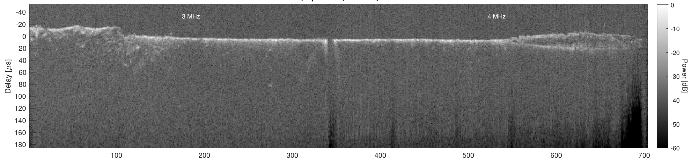
Orbit 22406, Cluttergram
