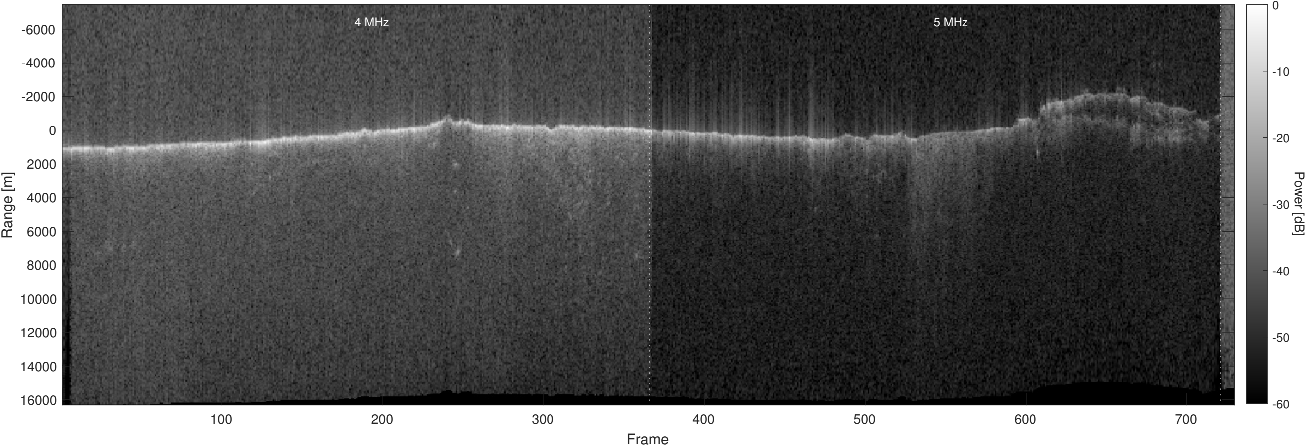
Orbit 22408, Optimized, No Window, Depth-Corrected, Channel 2
