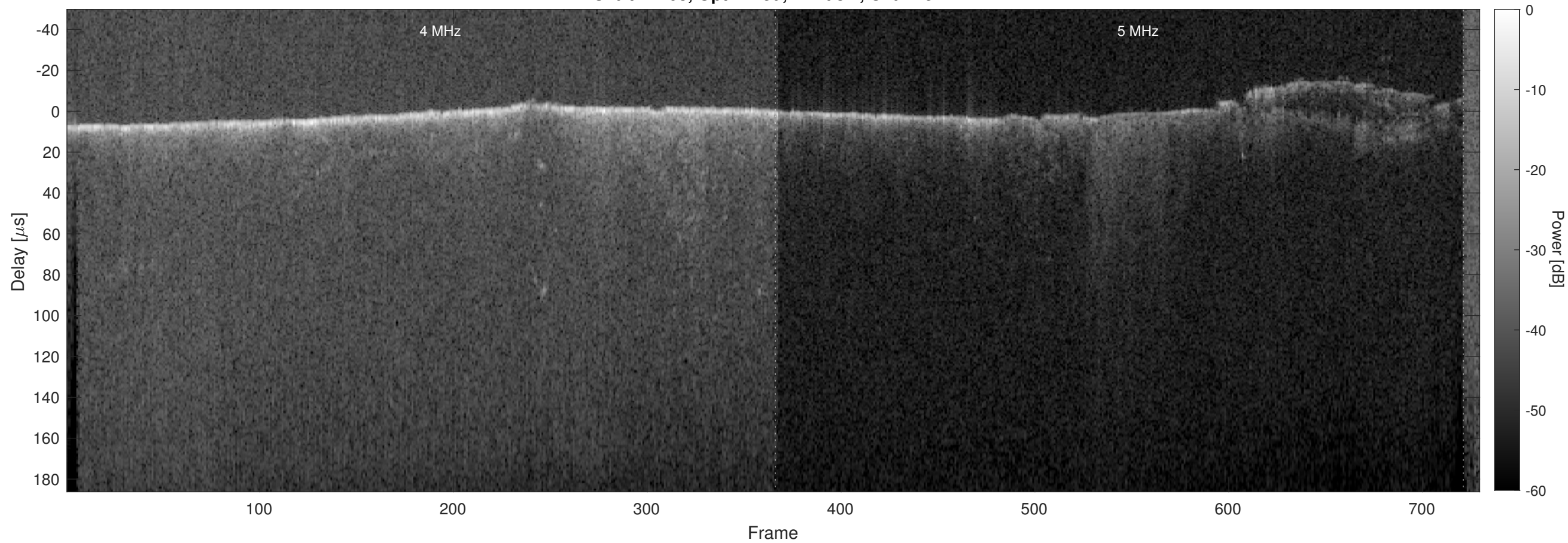
Orbit 22408, Optimized, Window, Channel 2
