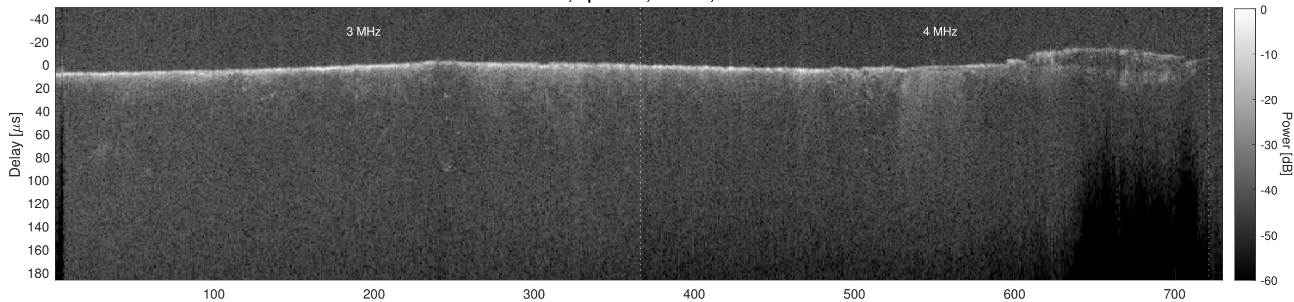
Orbit 22408, Cluttergram
