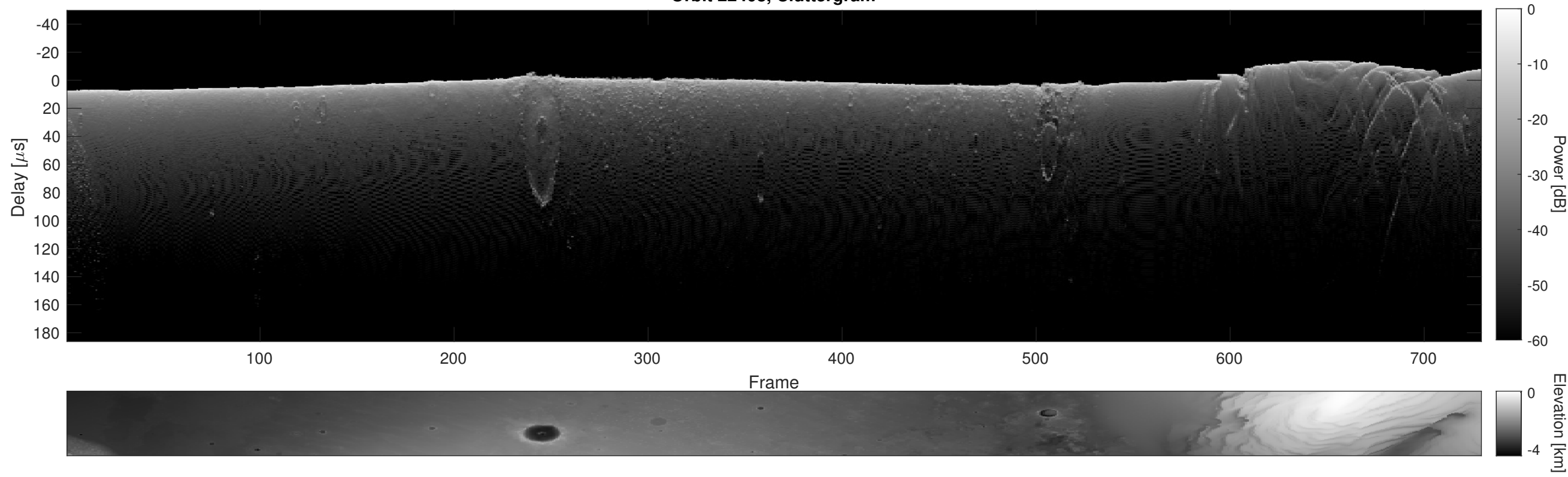
Orbit 22408, Cluttergram
