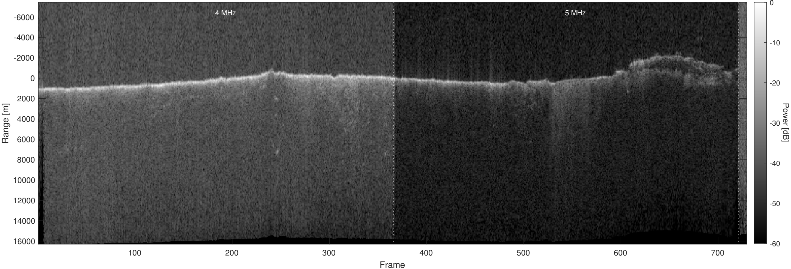
Orbit 22408, Optimized, Window, Depth-Corrected, Channel 2
