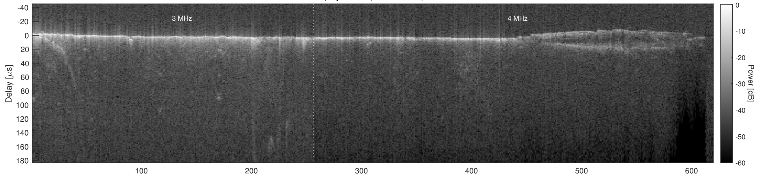
Orbit 22413, Cluttergram
