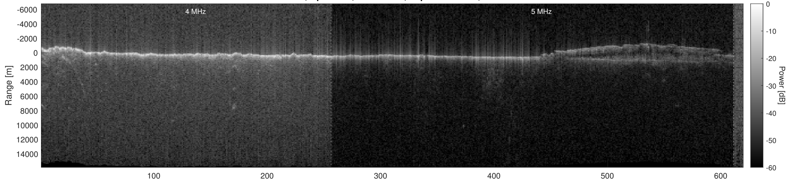
Orbit 22413, Optimized, No Window, Depth-Corrected, Channel 2
