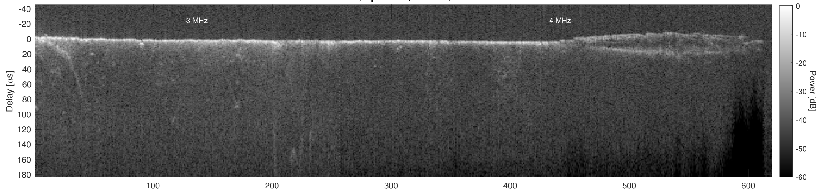
Orbit 22413, Cluttergram
