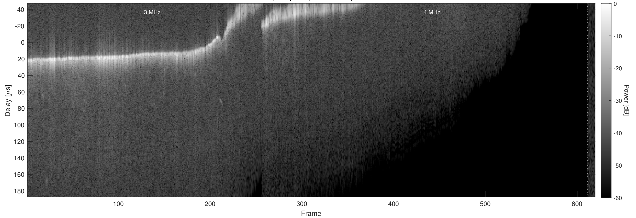
Orbit 22416, Chapman, No Window, Channel 2
