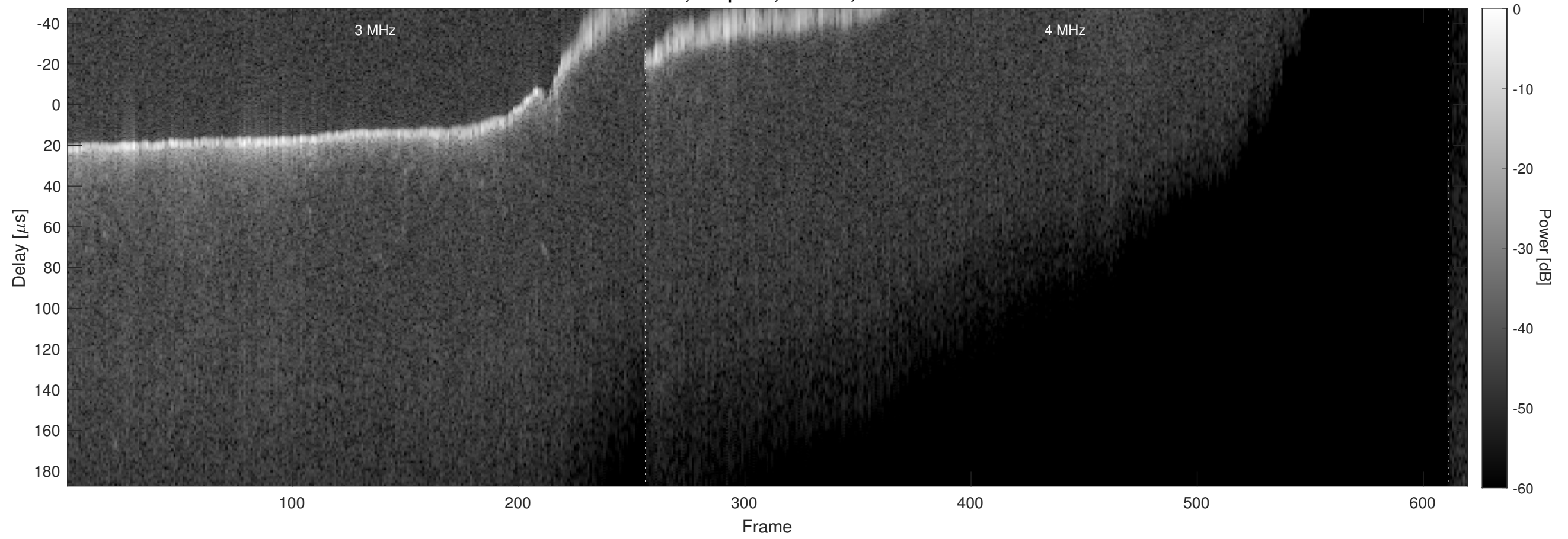
Orbit 22416, Chapman, Window, Channel 2
