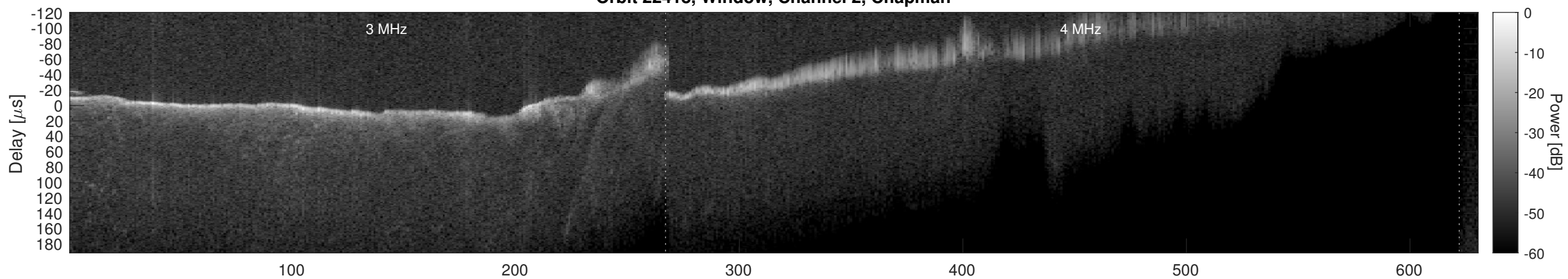
Orbit 22418, Window, Channel 2, Optimized
