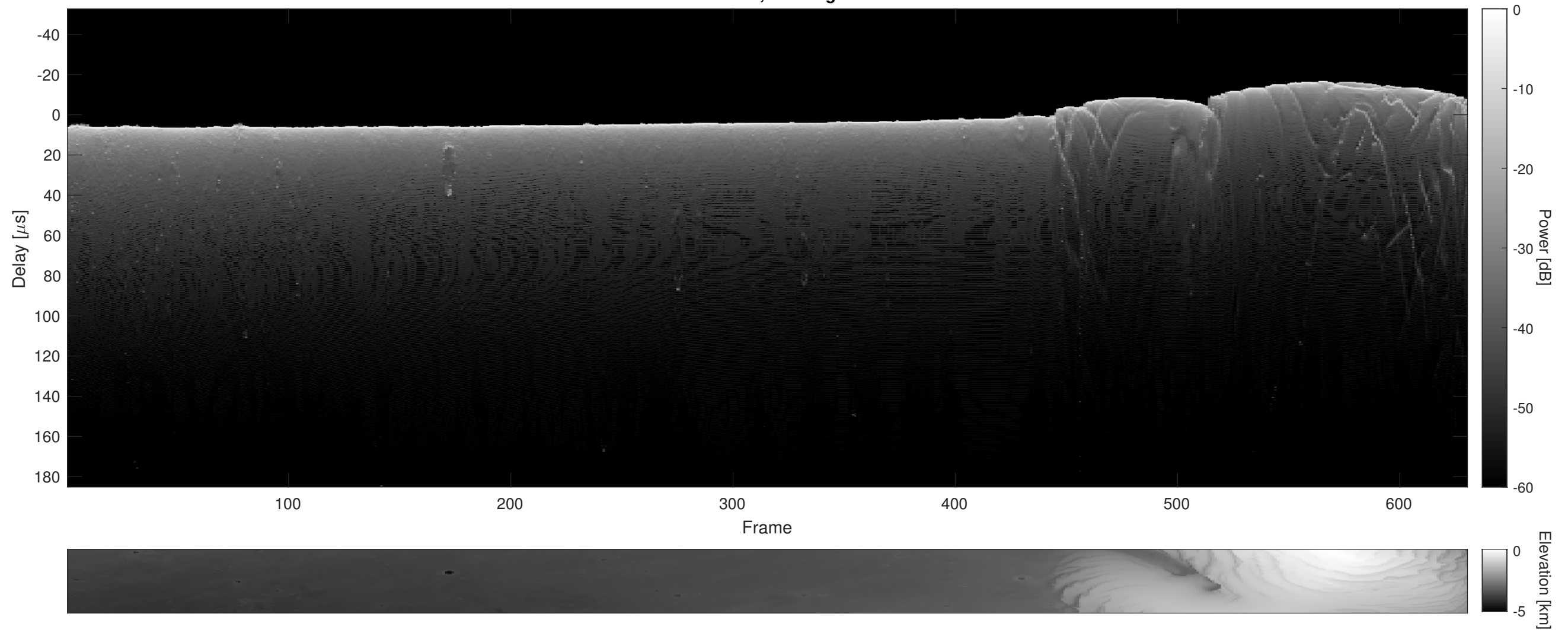
Orbit 22421, Cluttergram
