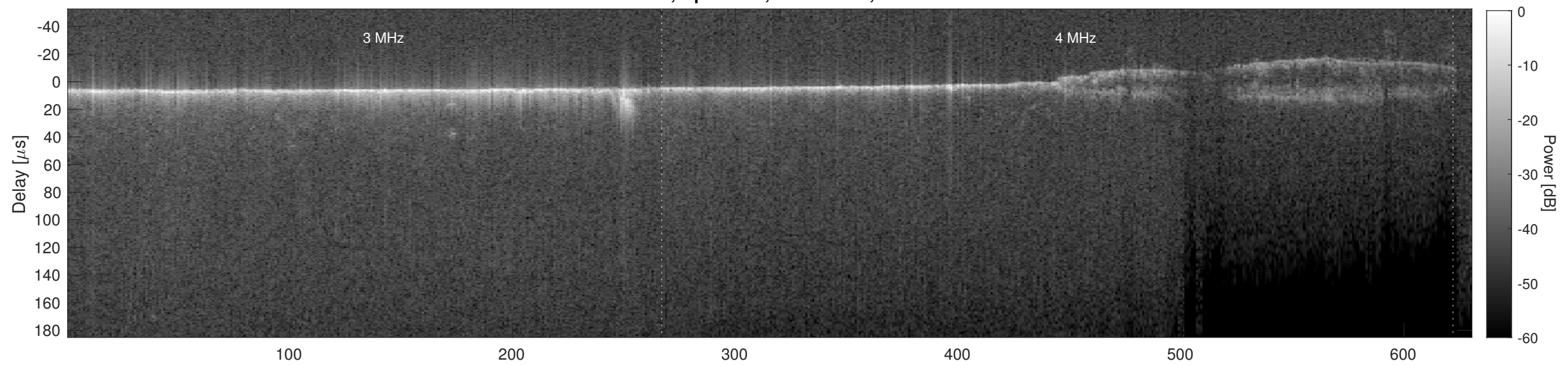
Orbit 22421, Cluttergram
