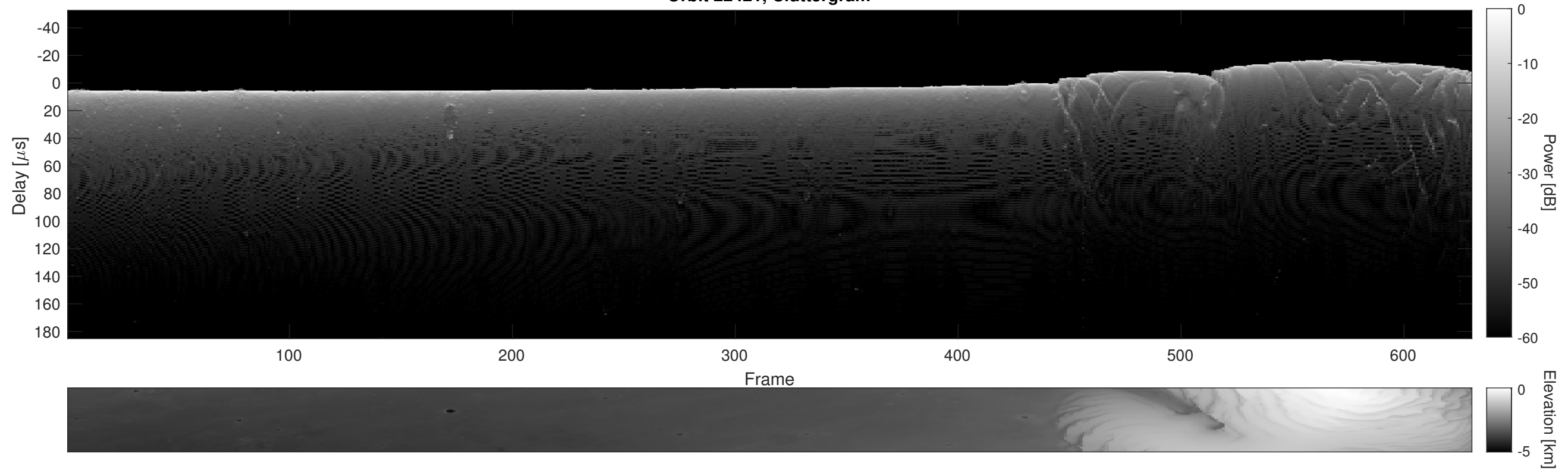
Orbit 22421, Cluttergram
