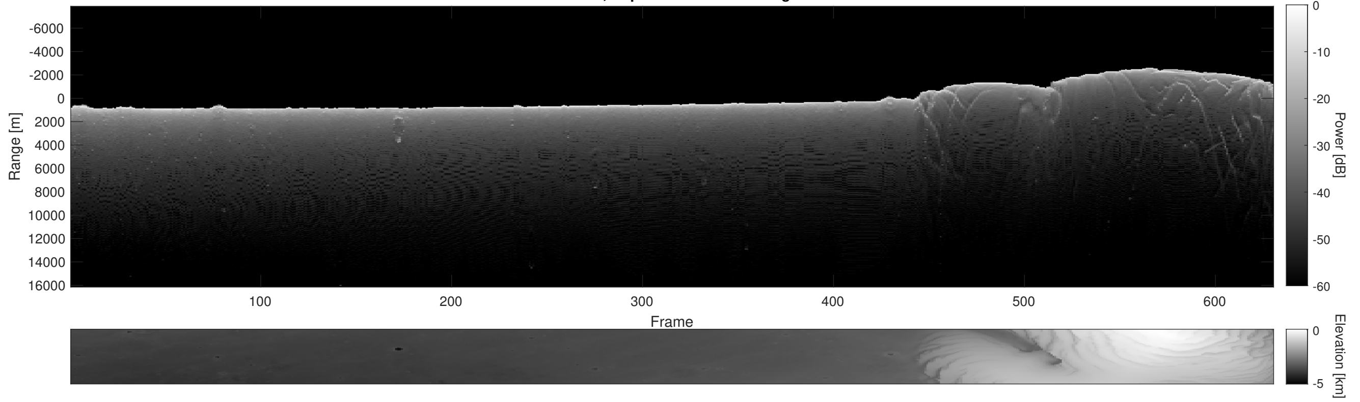
Orbit 22421, Depth-Corrected Cluttergram
