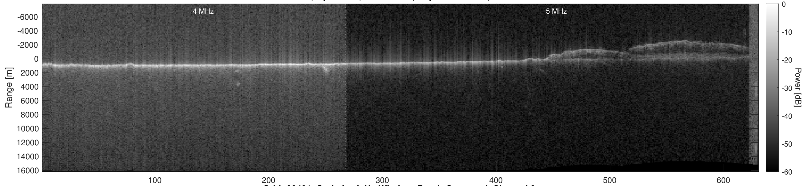
Orbit 22421, Optimized, No Window, Depth-Corrected, Channel 2
