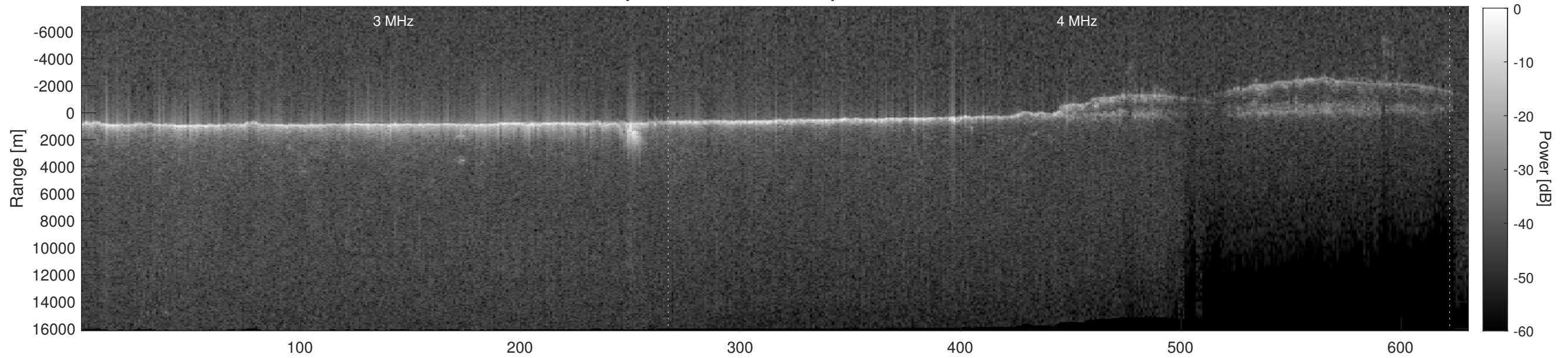
Orbit 22421, Depth-Corrected Cluttergram
