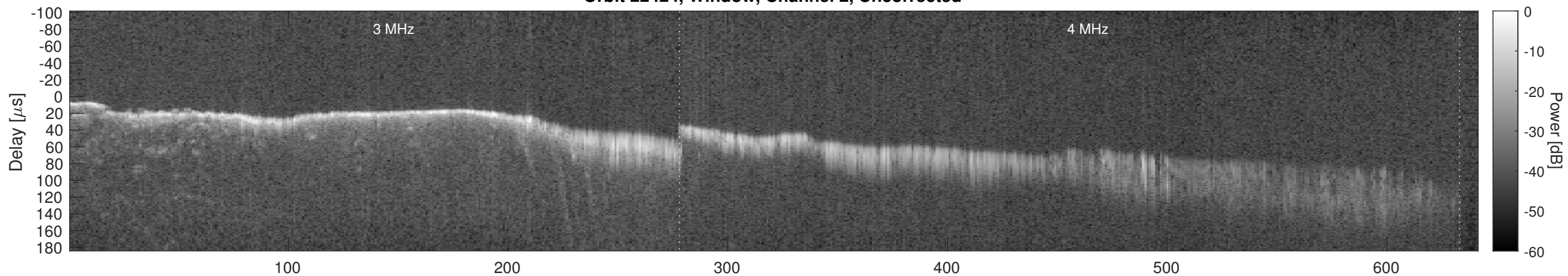
Orbit 22424, Window, Channel 2, Chapman
