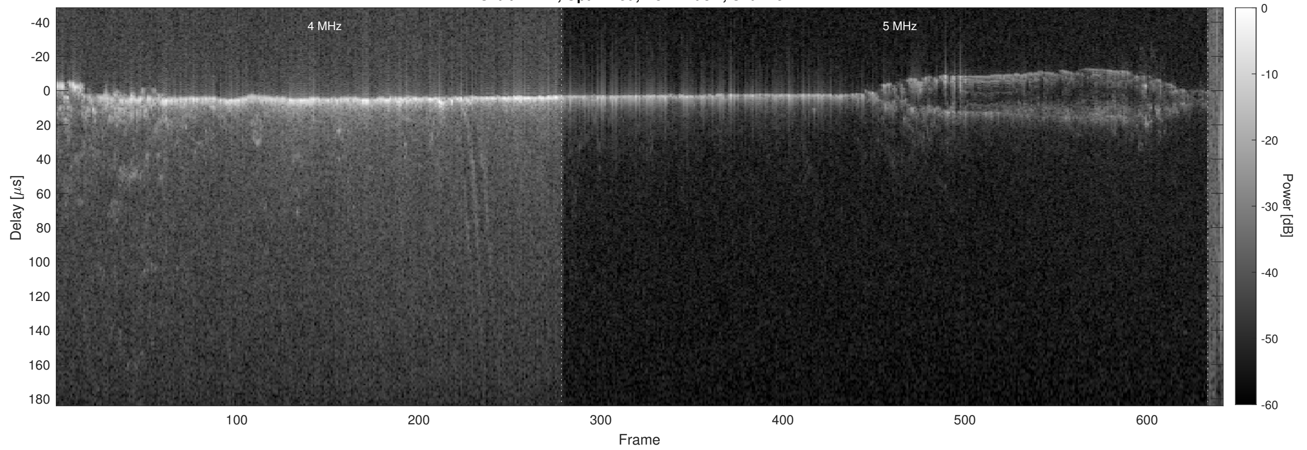
Orbit 22424, Optimized, No Window, Channel 2
