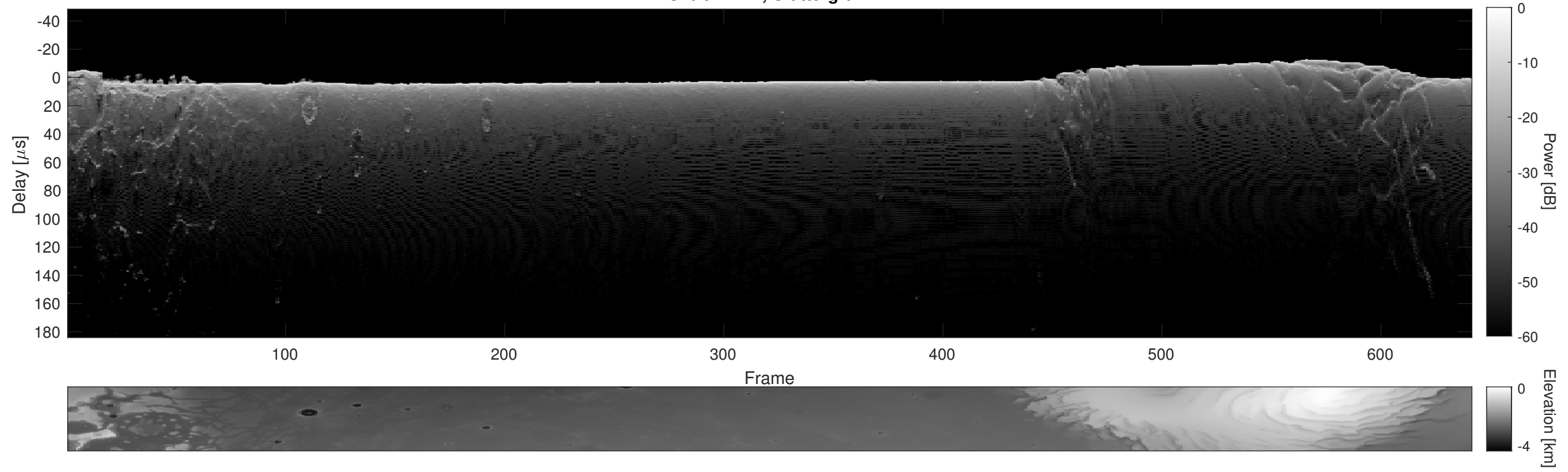
Orbit 22424, Cluttergram
