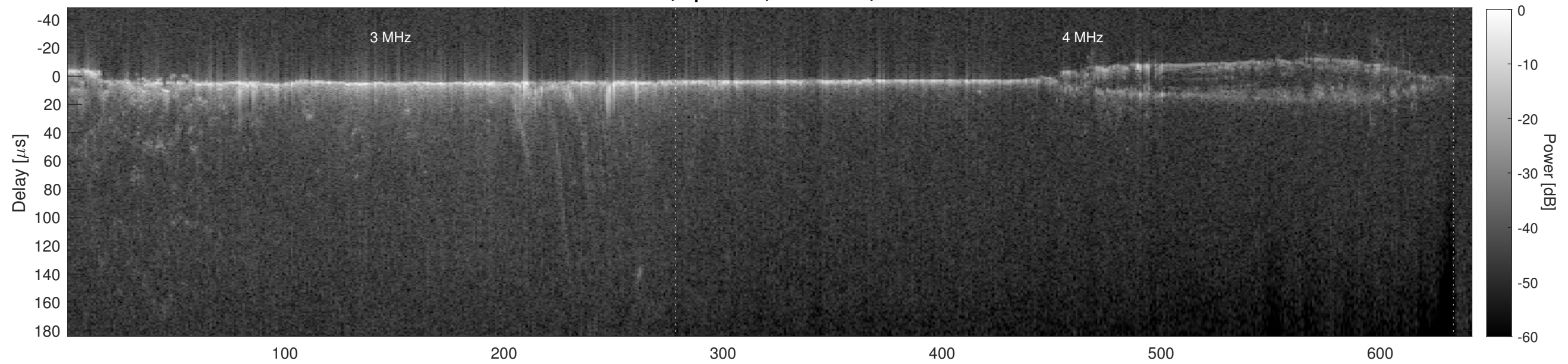
Orbit 22424, Cluttergram
