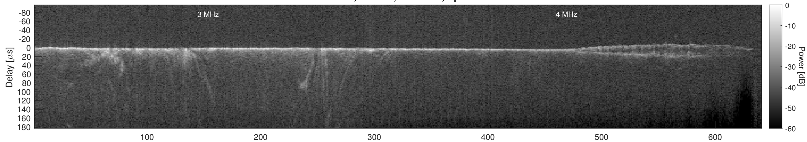
Orbit 22427, Cluttergram
