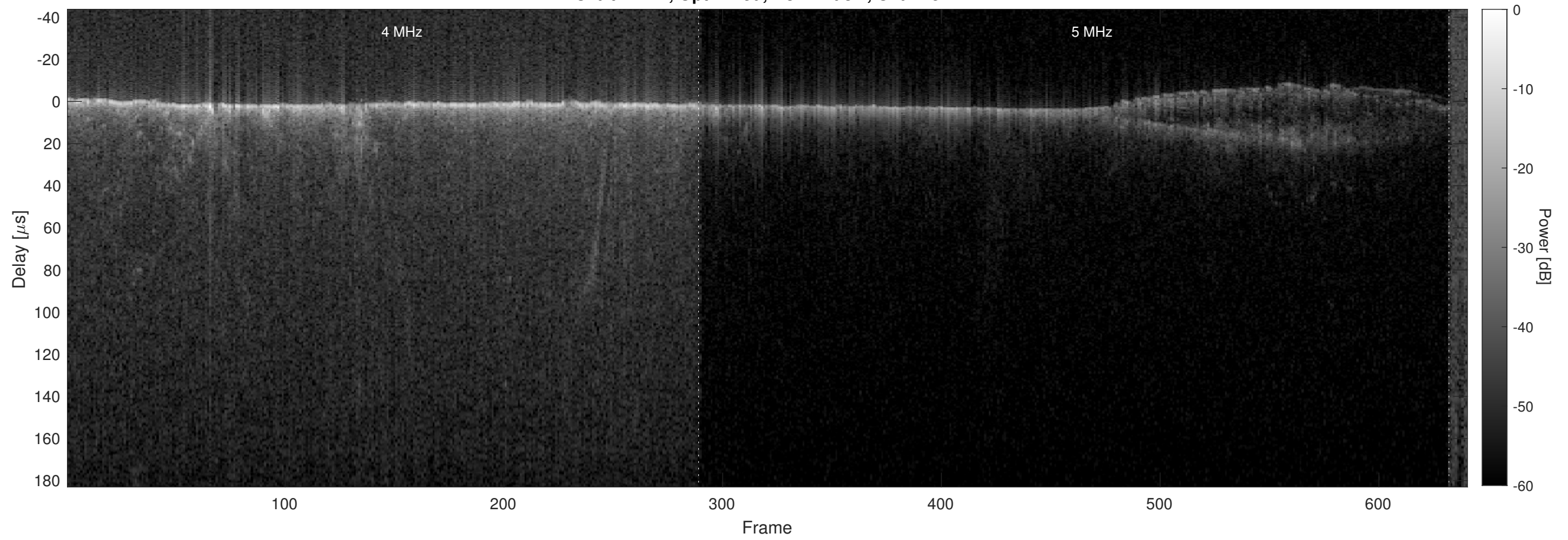
Orbit 22427, Optimized, No Window, Channel 2
