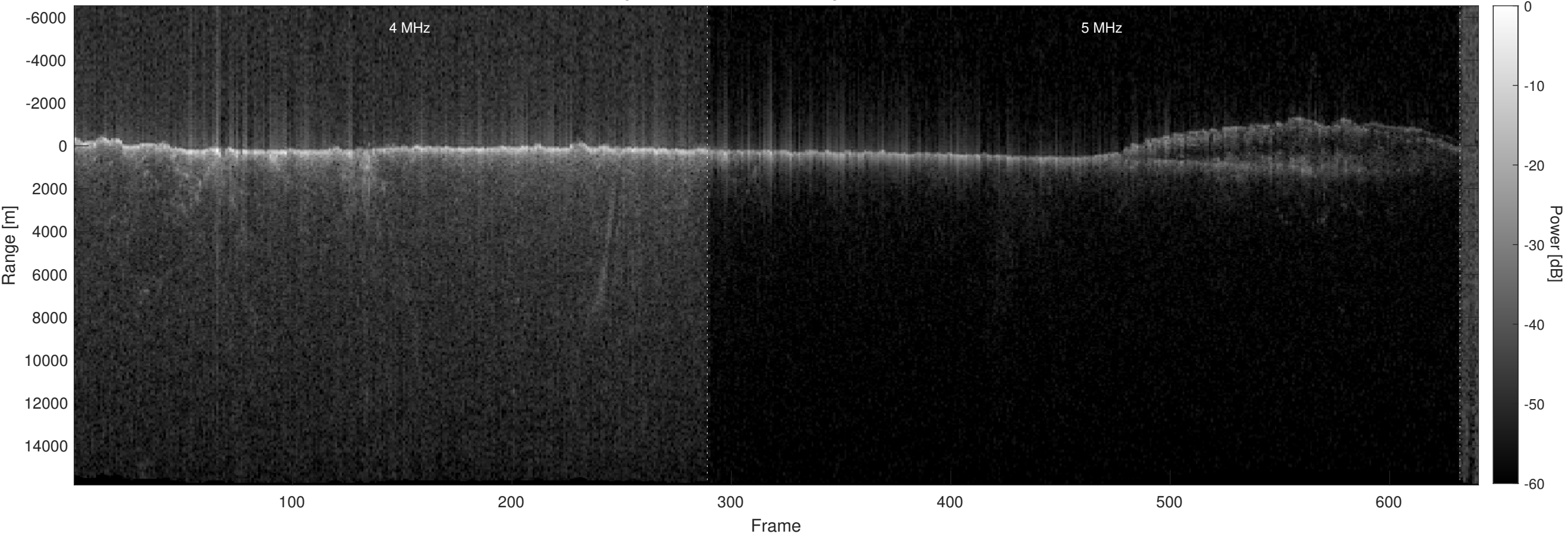
Orbit 22427, Optimized, No Window, Depth-Corrected, Channel 2
