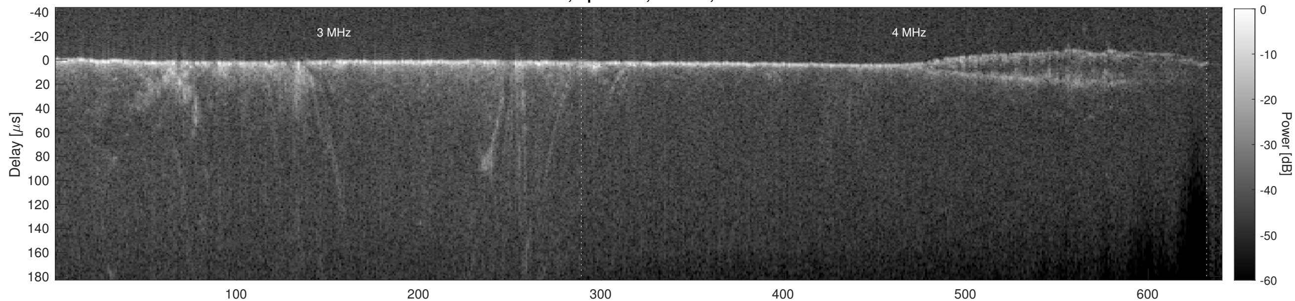
Orbit 22427, Cluttergram
