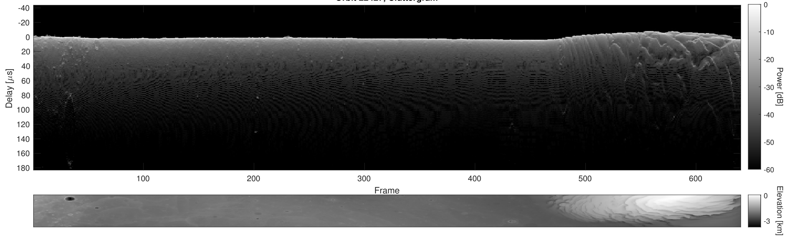
Orbit 22427, Cluttergram
