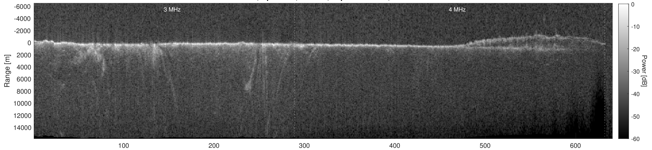
Orbit 22427, Depth-Corrected Cluttergram
