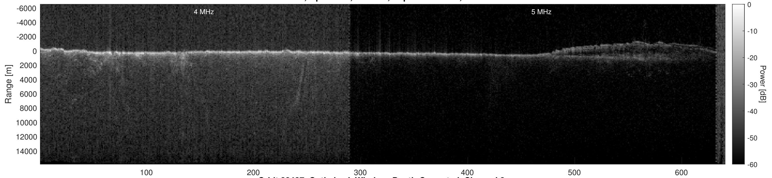
Orbit 22427, Optimized, Window, Depth-Corrected, Channel 2
