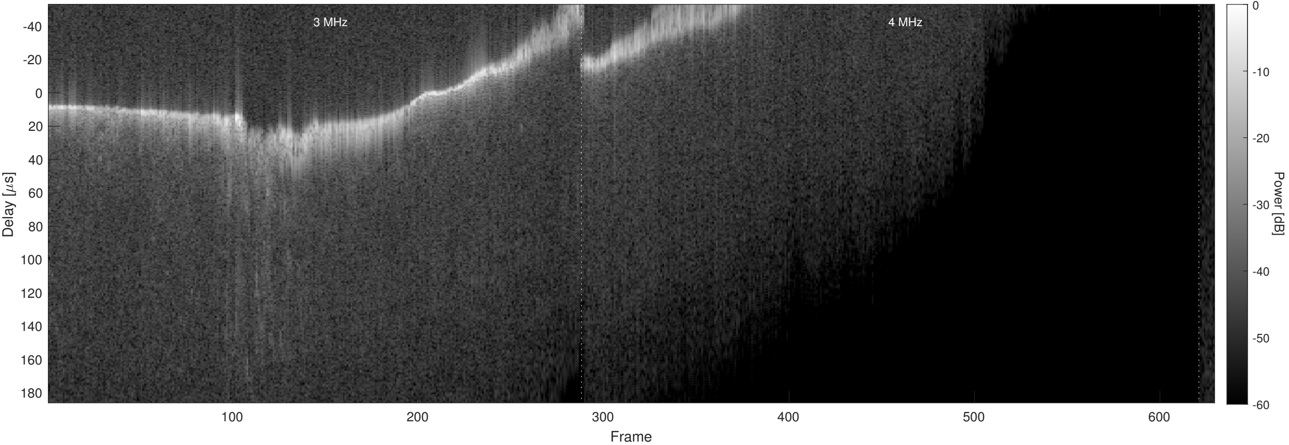
Orbit 22428, Chapman, No Window, Channel 2
