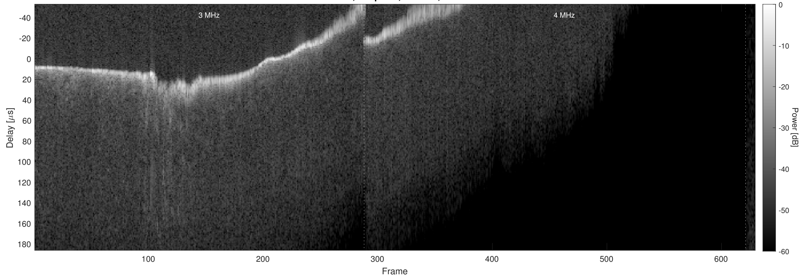
Orbit 22428, Chapman, Window, Channel 2
