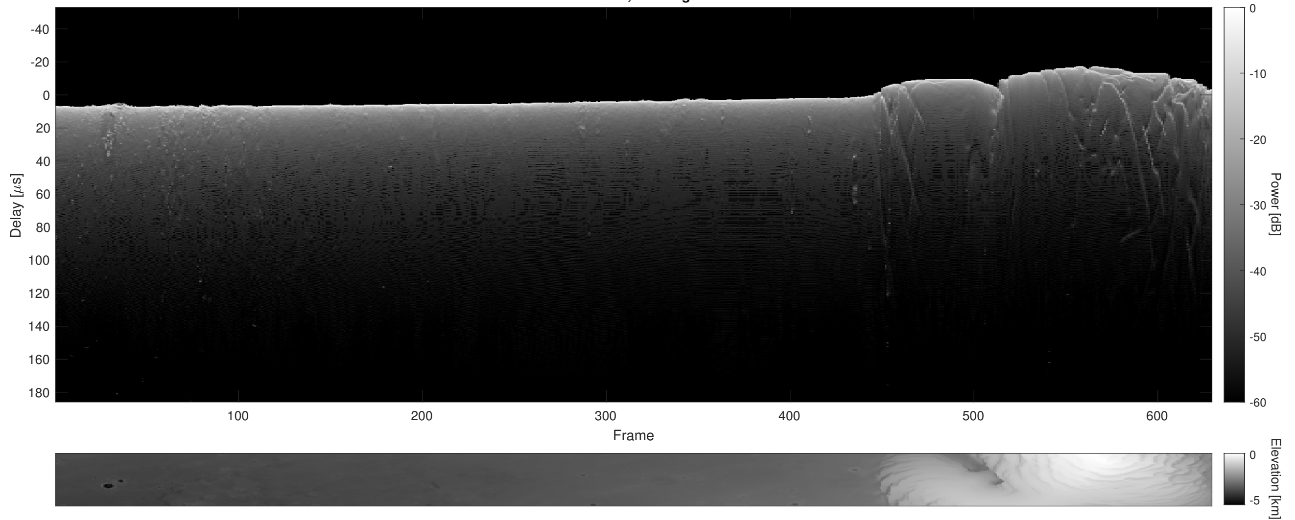
Orbit 22428, Cluttergram
