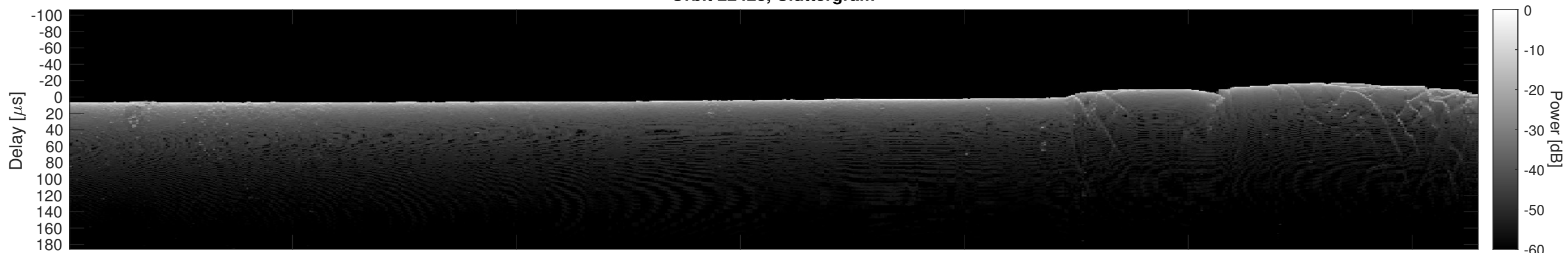
Orbit 22428, Cluttergram
