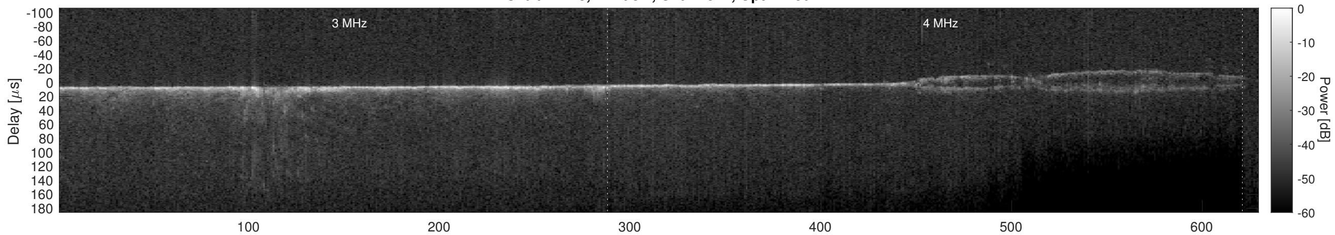
Orbit 22428, Cluttergram
