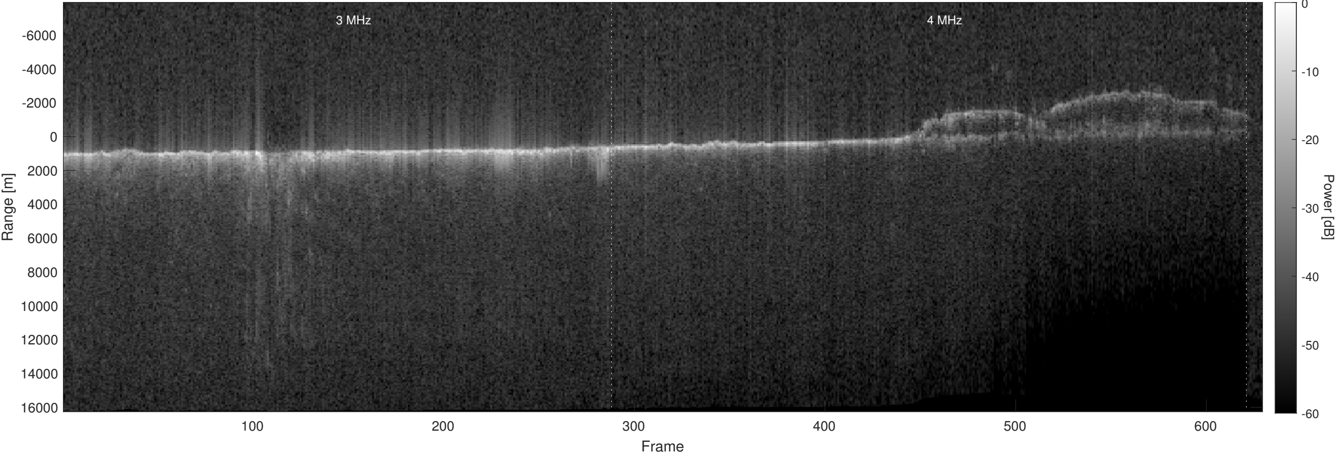
Orbit 22428, Optimized, No Window, Depth-Corrected, Channel 2
