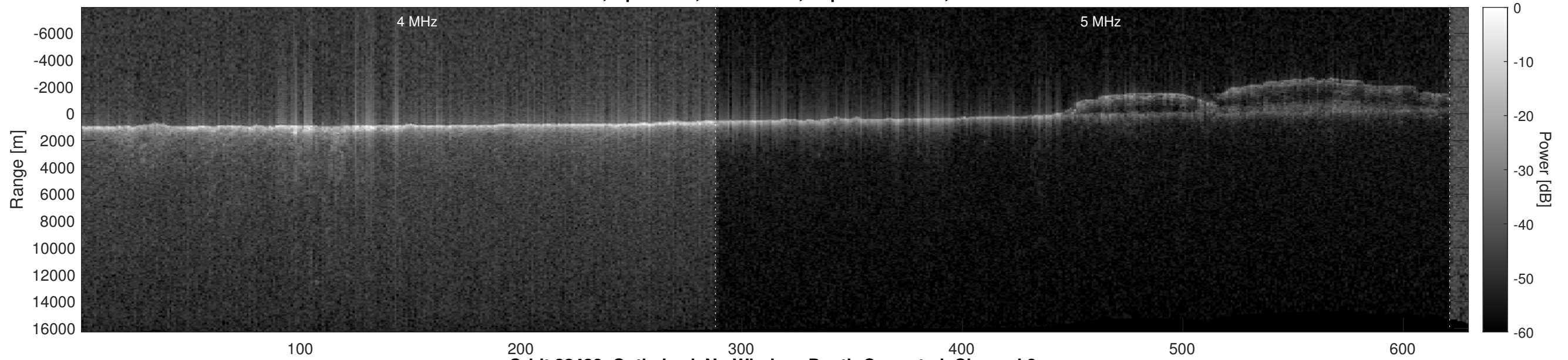
Orbit 22428, Optimized, No Window, Depth-Corrected, Channel 2
