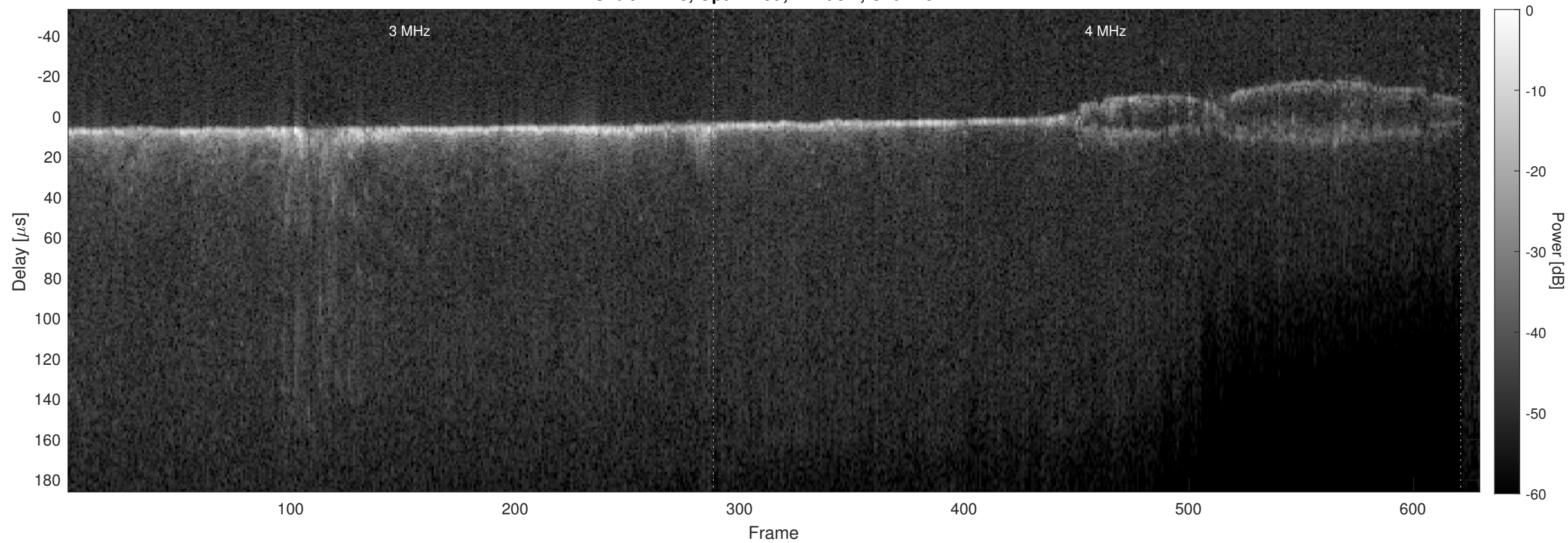
Orbit 22428, Optimized, Window, Channel 2
