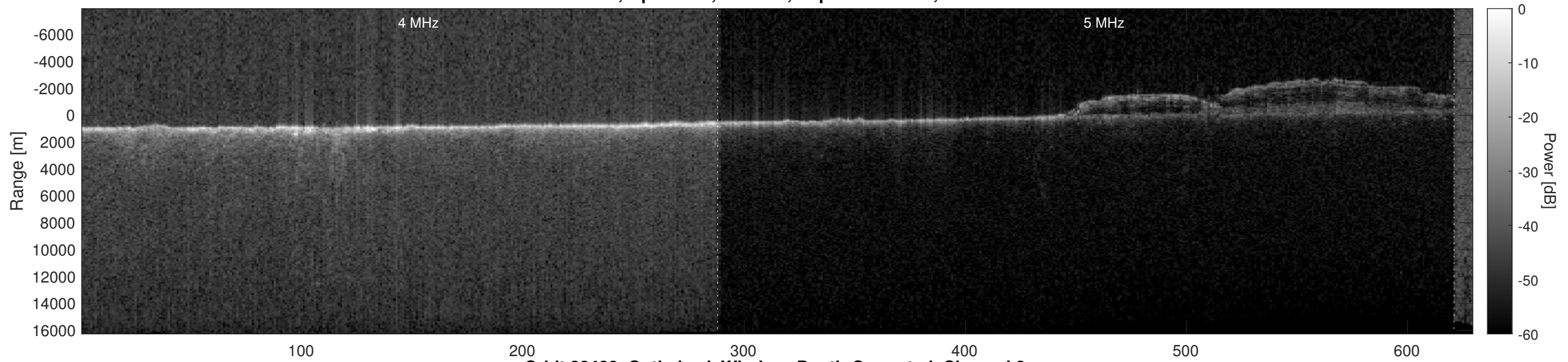
Orbit 22428, Optimized, Window, Depth-Corrected, Channel 2
