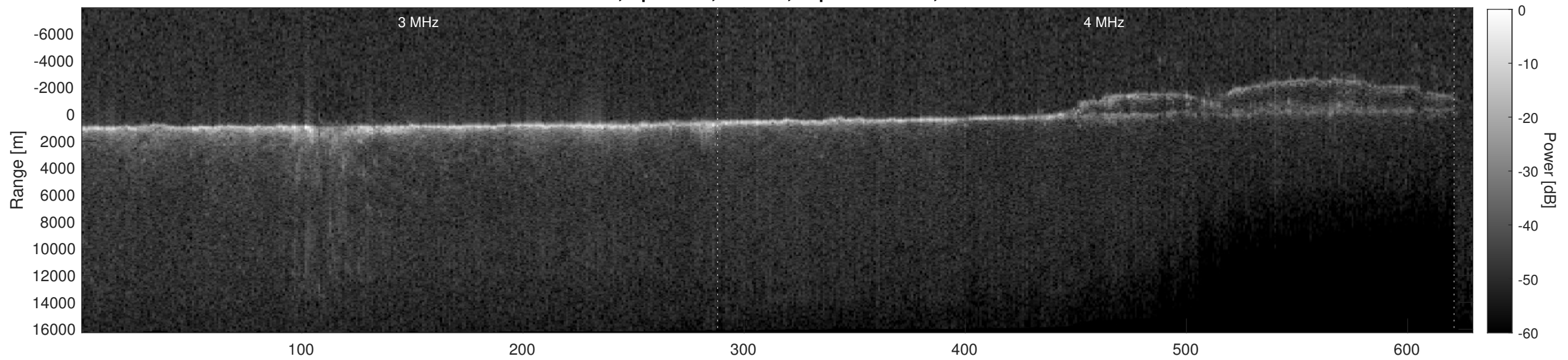
Orbit 22428, Depth-Corrected Cluttergram
