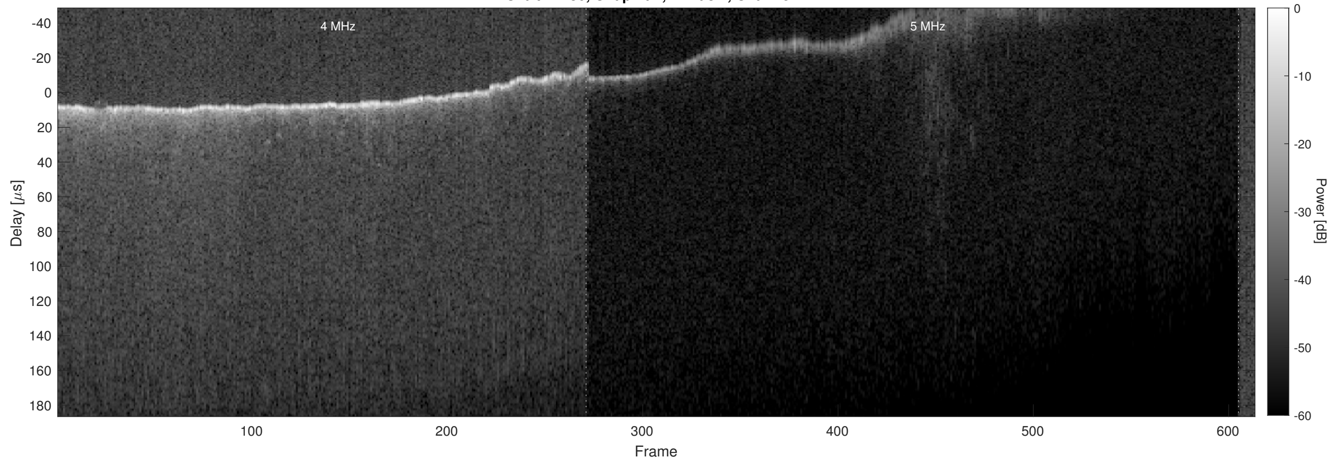
Orbit 22430, Chapman, Window, Channel 2
