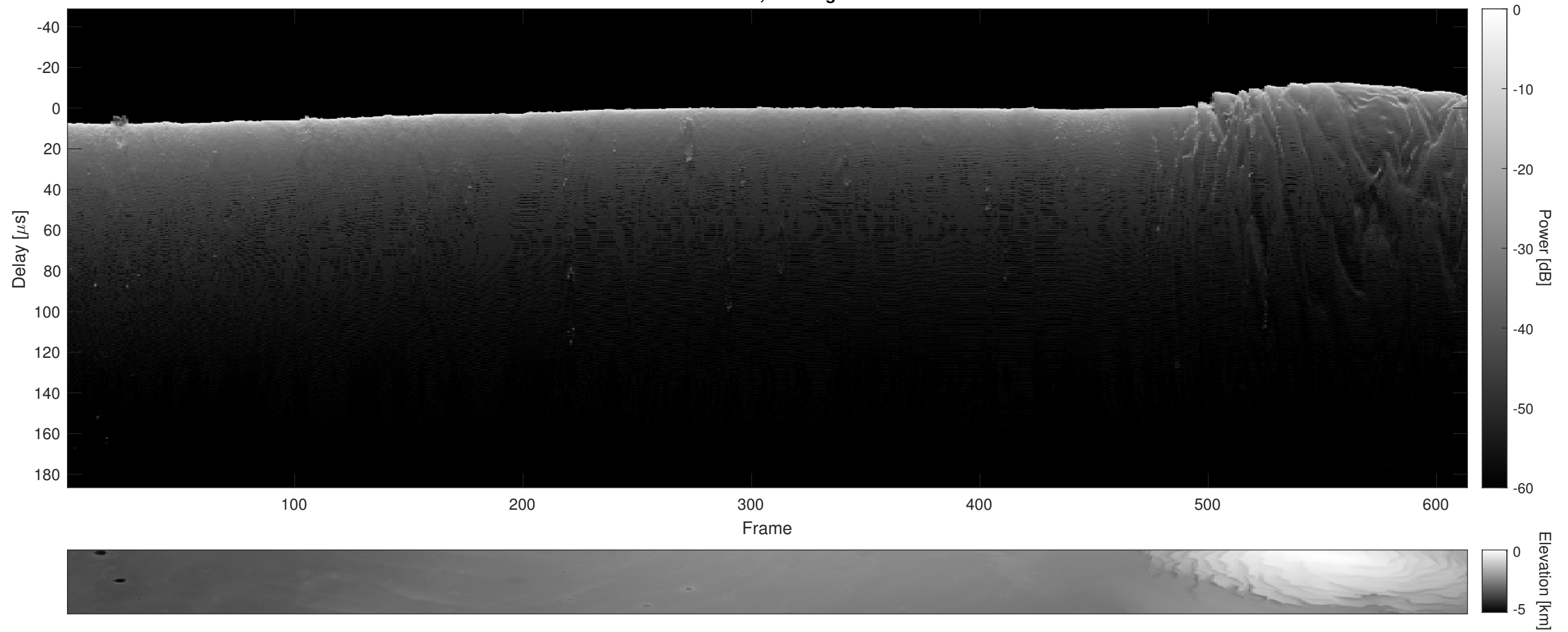
Orbit 22430, Cluttergram
