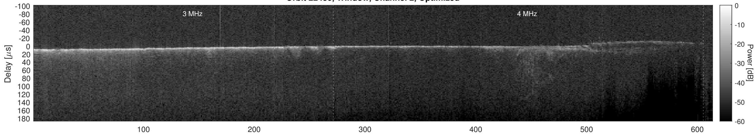
Orbit 22430, Cluttergram
