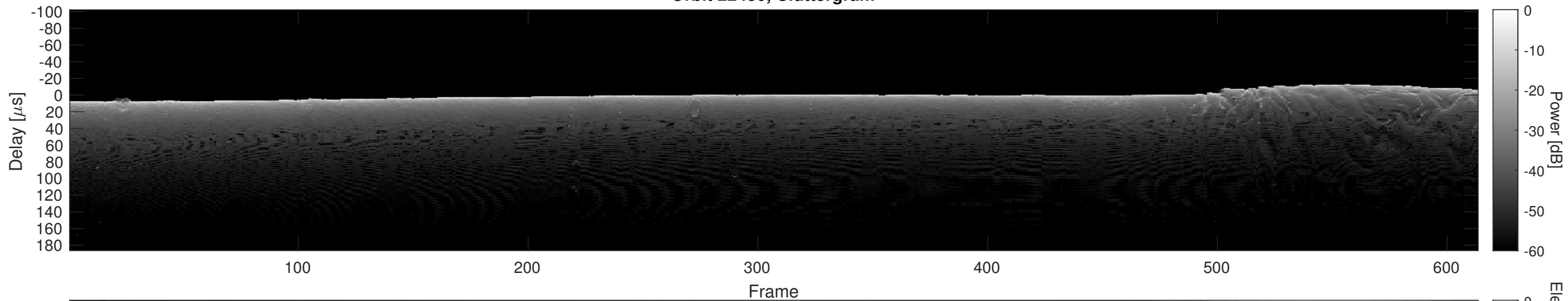
Orbit 22430, Cluttergram
