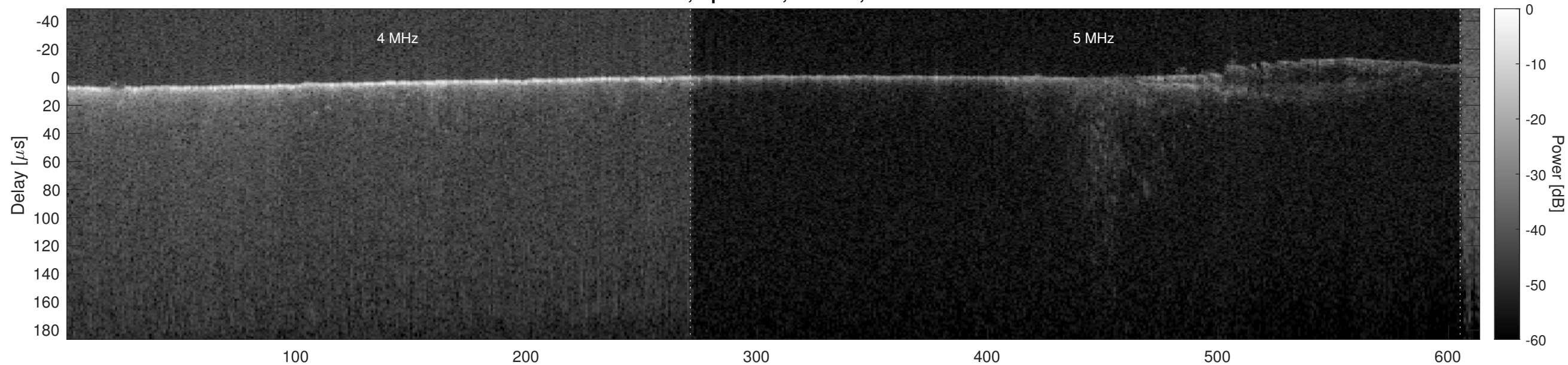
Orbit 22430, Optimized, Window, Channel 2
