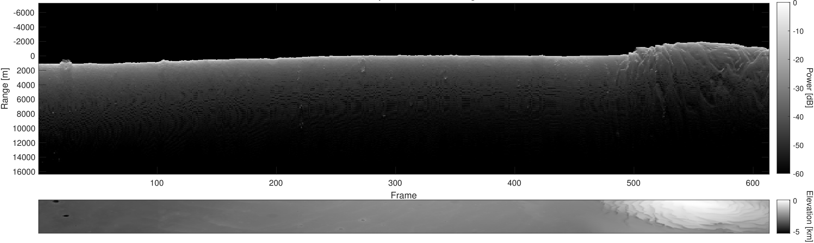
Orbit 22430, Depth-Corrected Cluttergram
