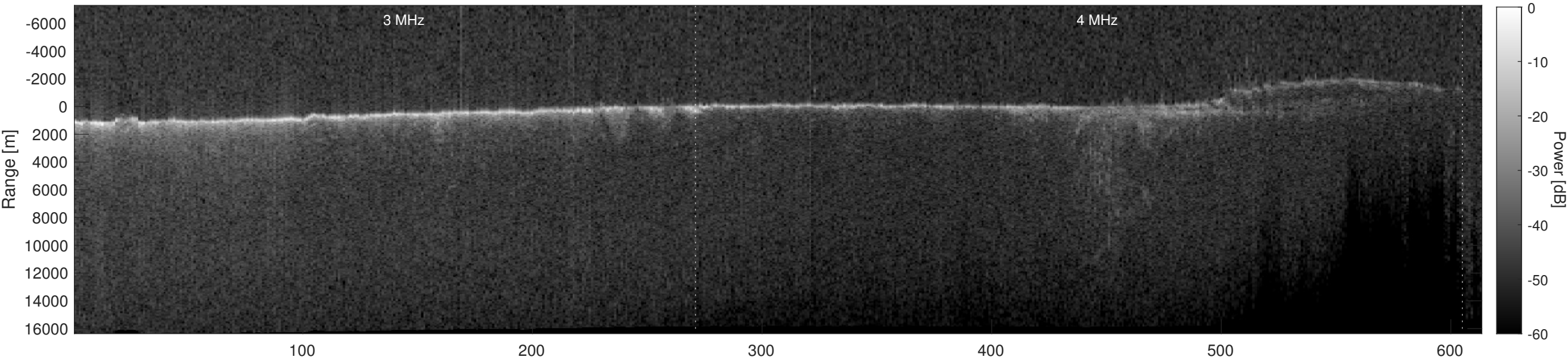
Orbit 22430, Depth-Corrected Cluttergram
