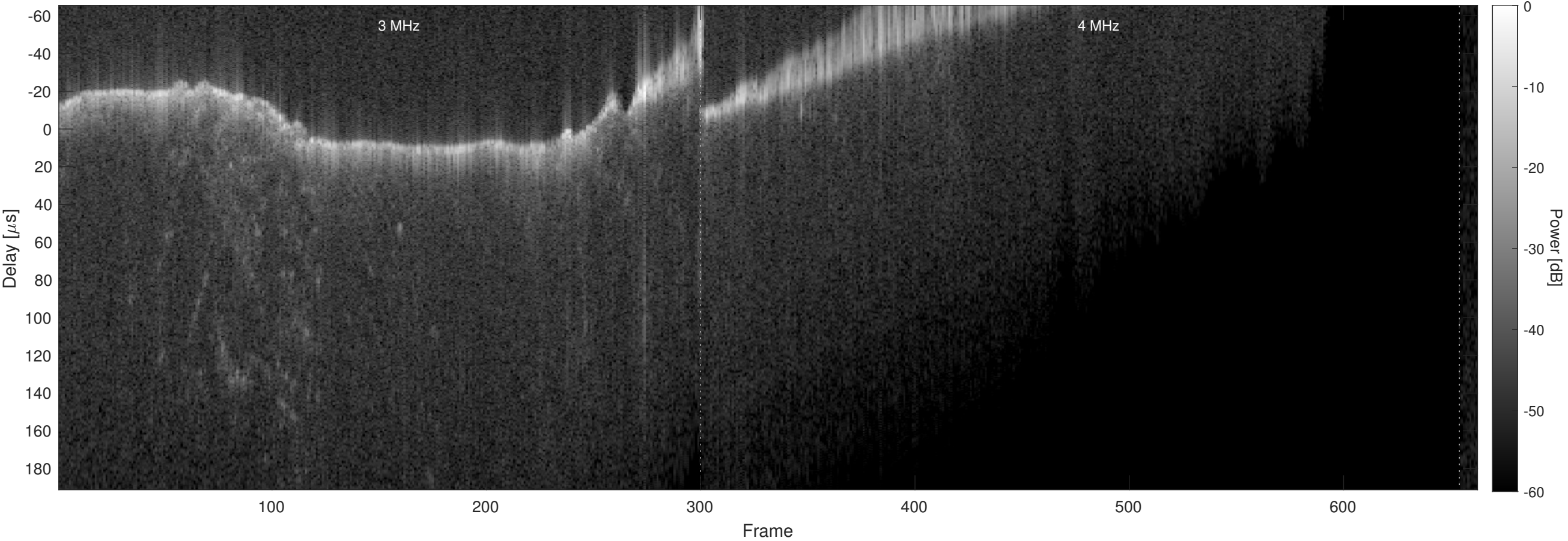
Orbit 22432, Chapman, No Window, Channel 2
