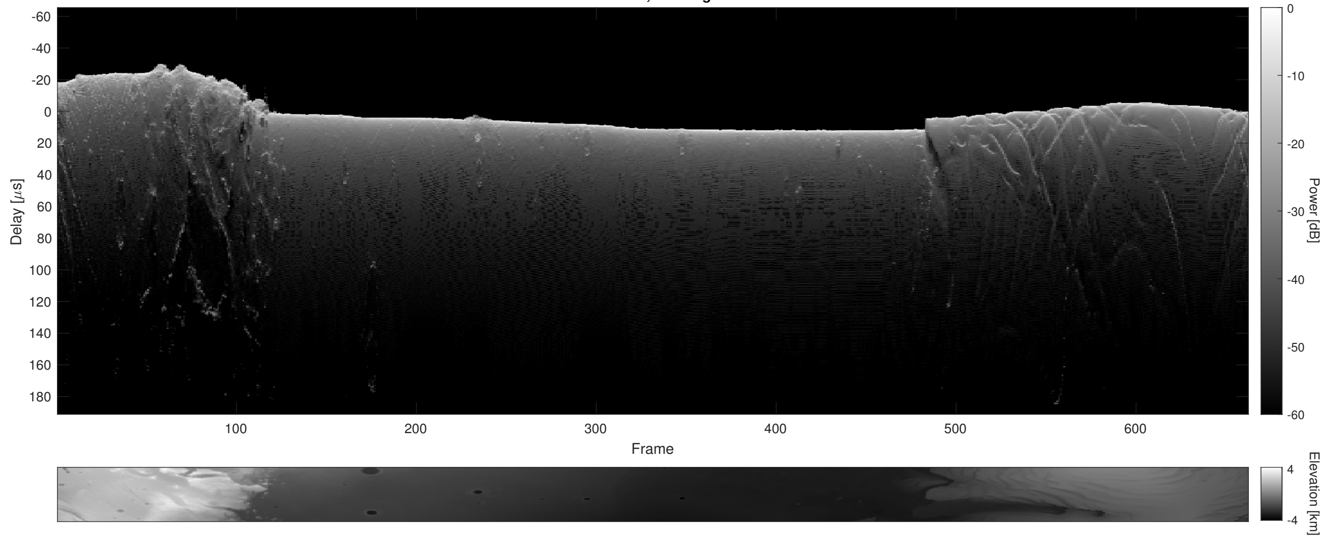
Orbit 22432, Cluttergram
