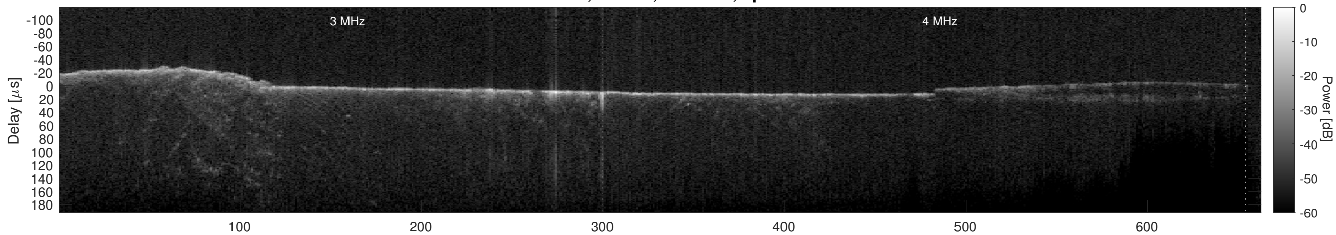
Orbit 22432, Cluttergram
