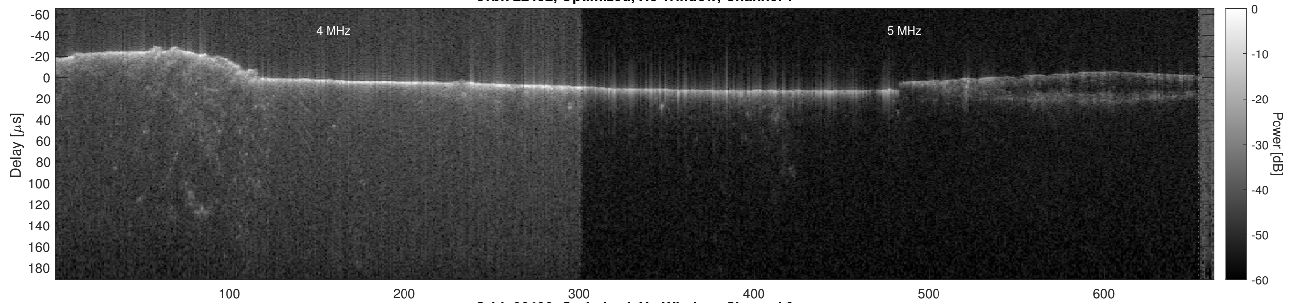
Orbit 22432, Optimized, No Window, Channel 2
