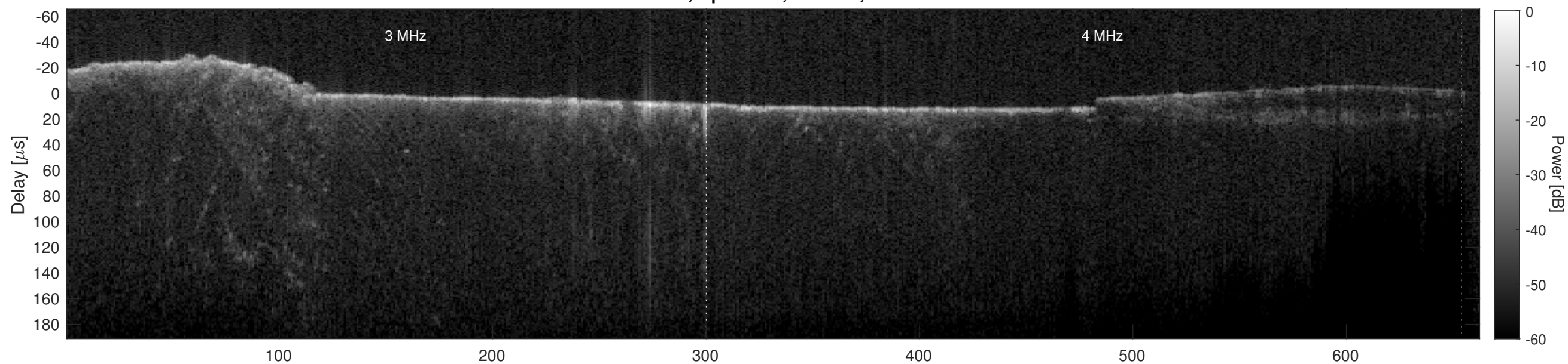
Orbit 22432, Cluttergram
