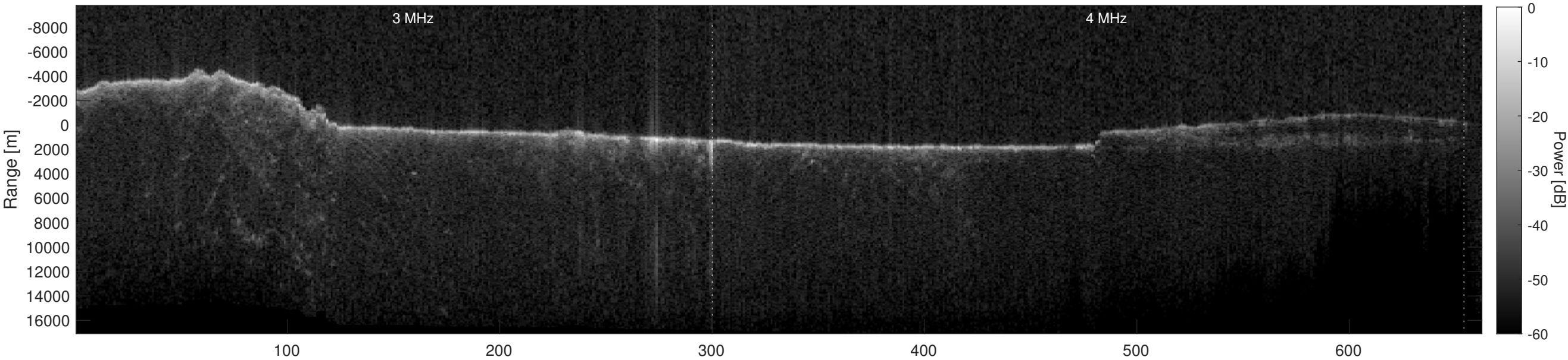
Orbit 22432, Depth-Corrected Cluttergram
