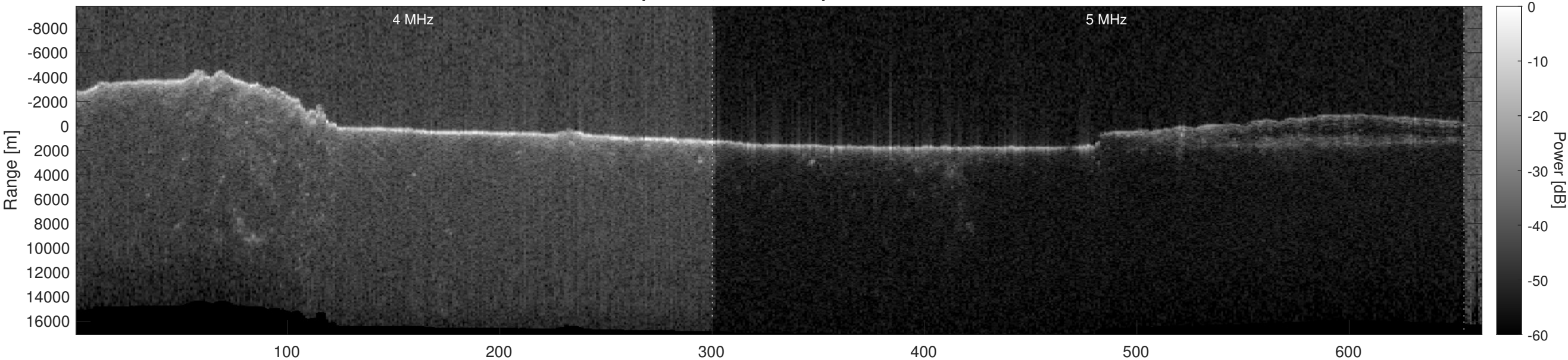
Orbit 22432, Optimized, Window, Depth-Corrected, Channel 2
