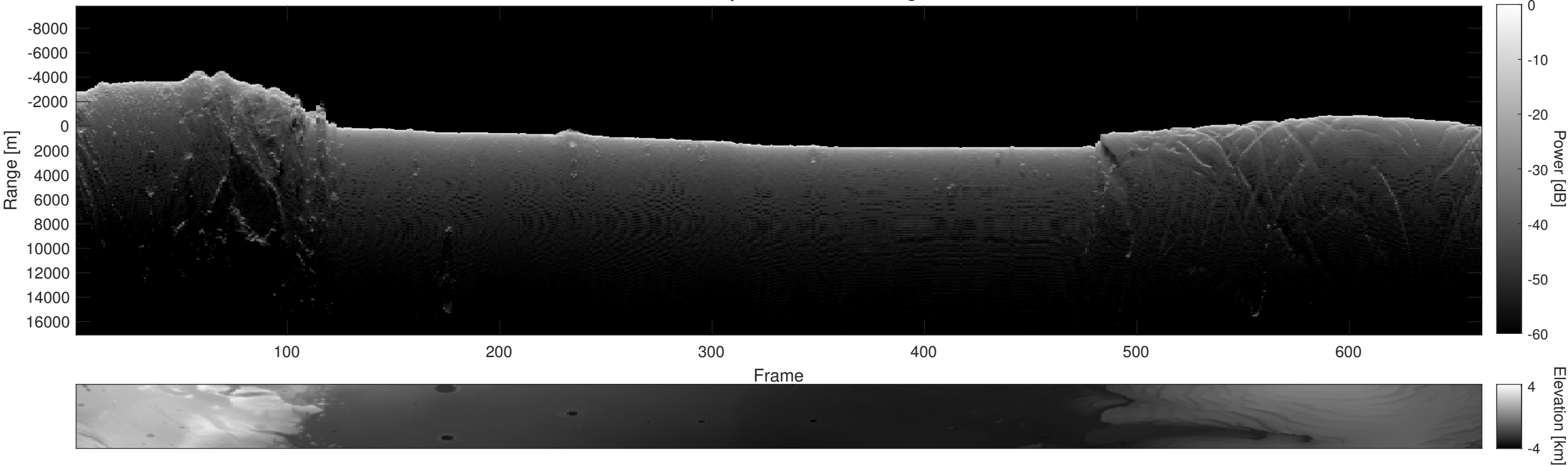
Orbit 22432, Depth-Corrected Cluttergram
