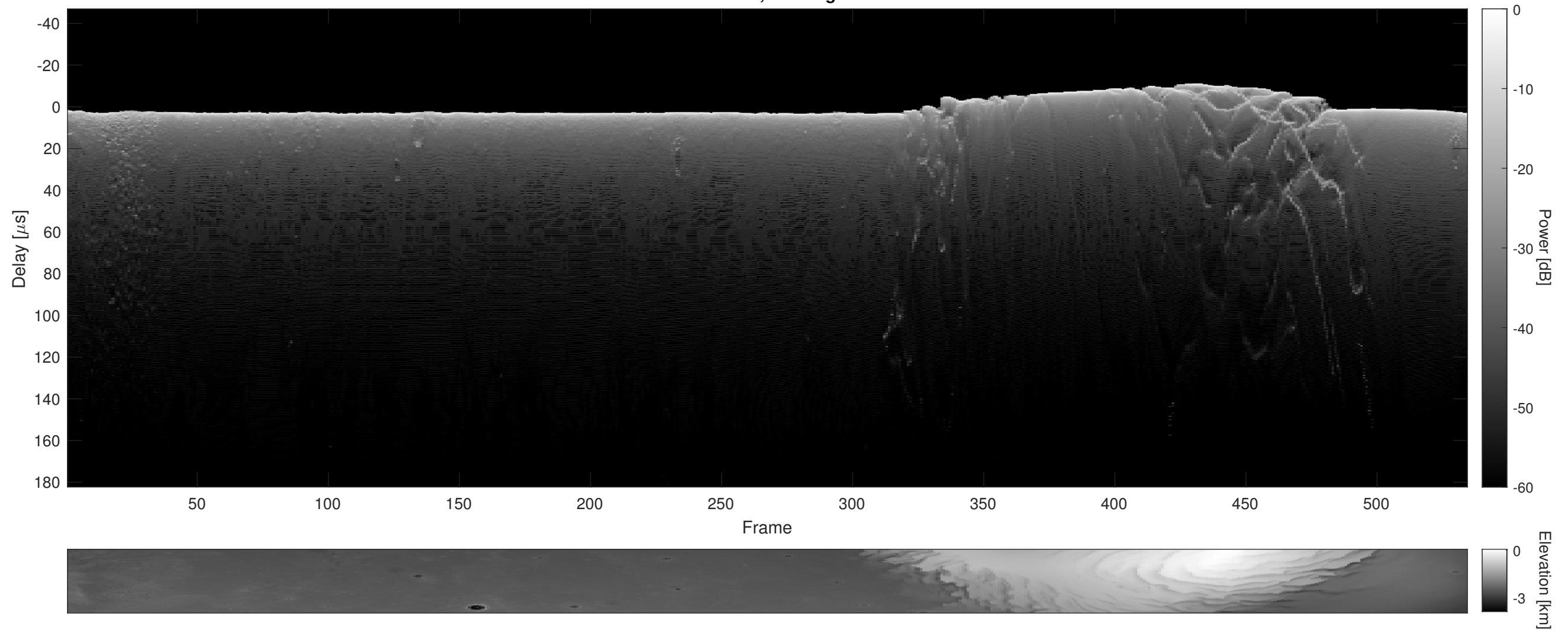
Orbit 22512, Cluttergram
