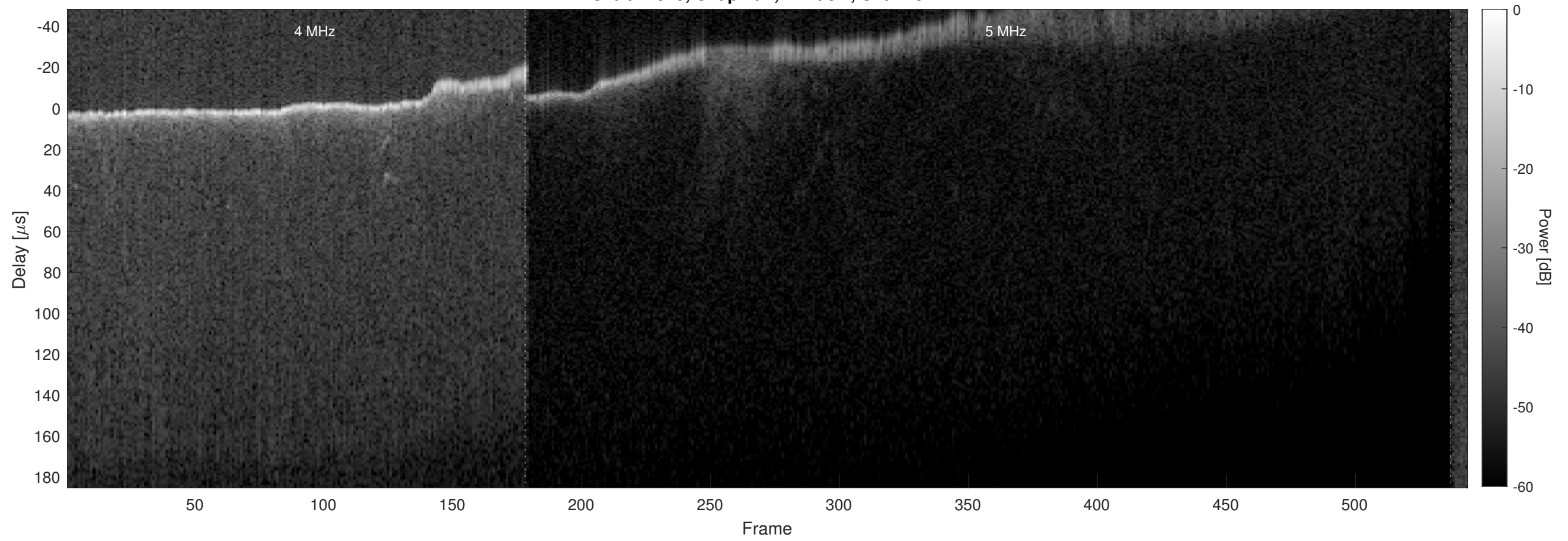
Orbit 22513, Chapman, Window, Channel 2
