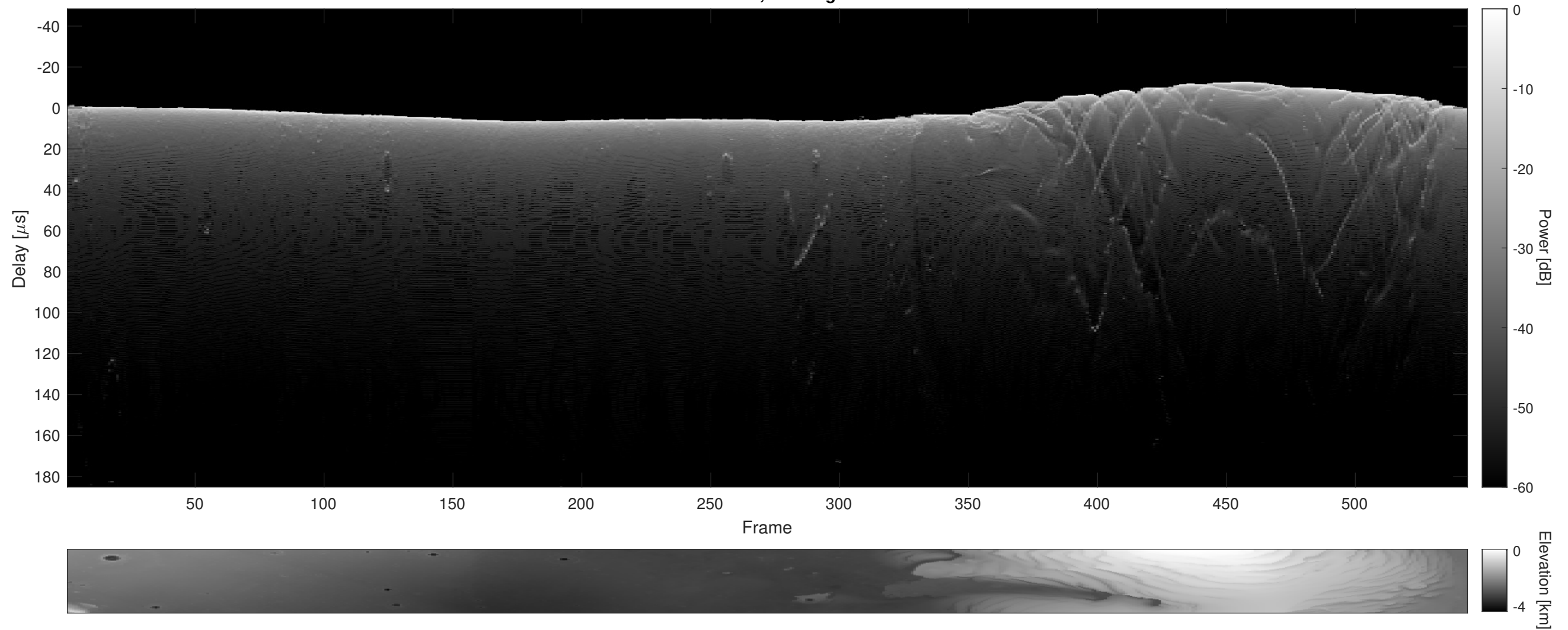
Orbit 22513, Cluttergram
