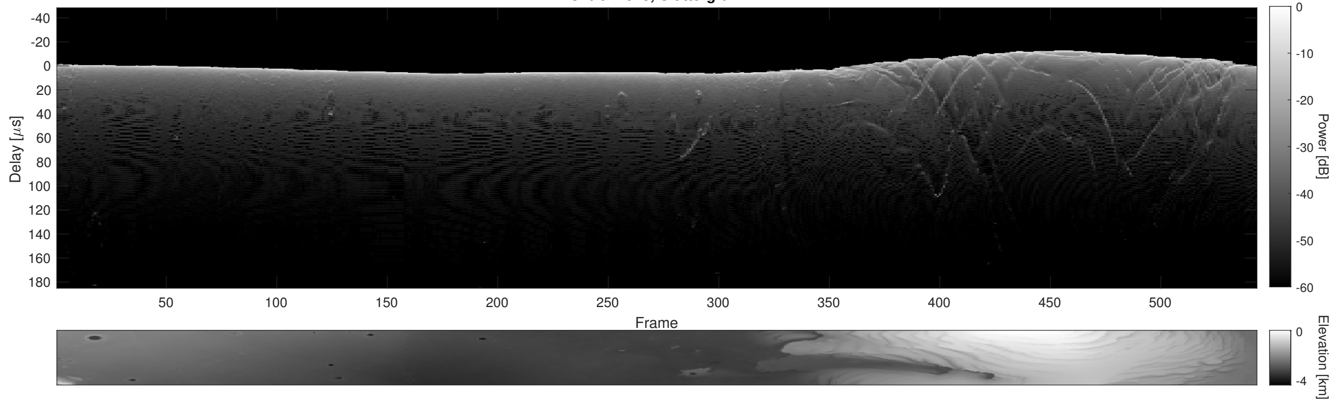
Orbit 22513, Cluttergram
