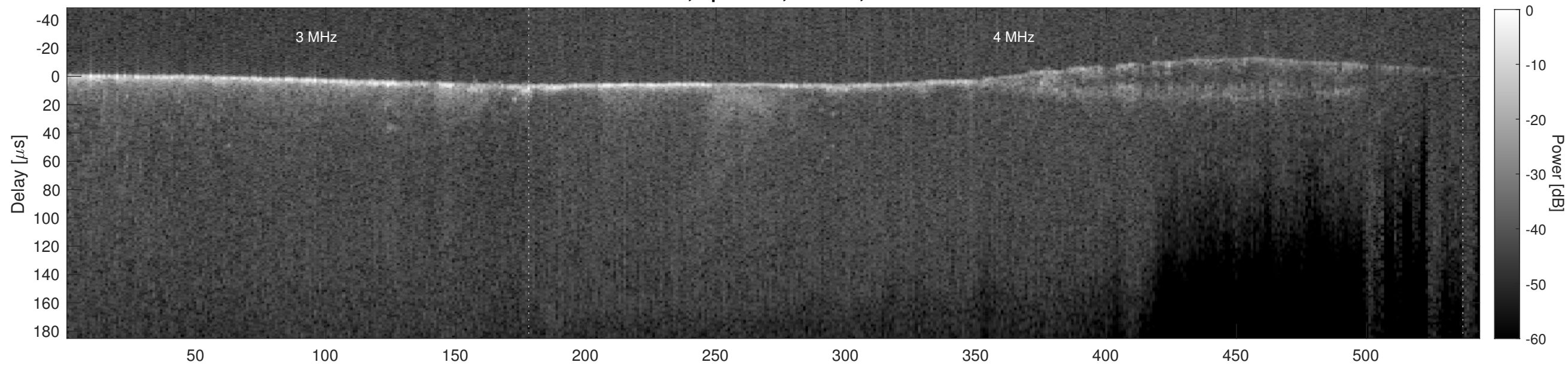
Orbit 22513, Cluttergram
