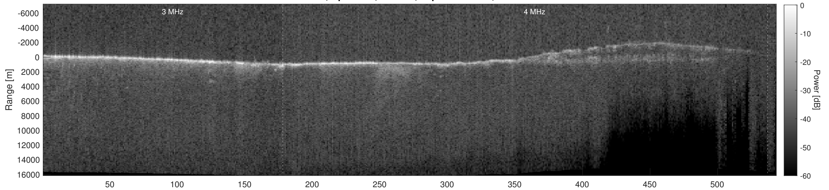
Orbit 22513, Depth-Corrected Cluttergram
