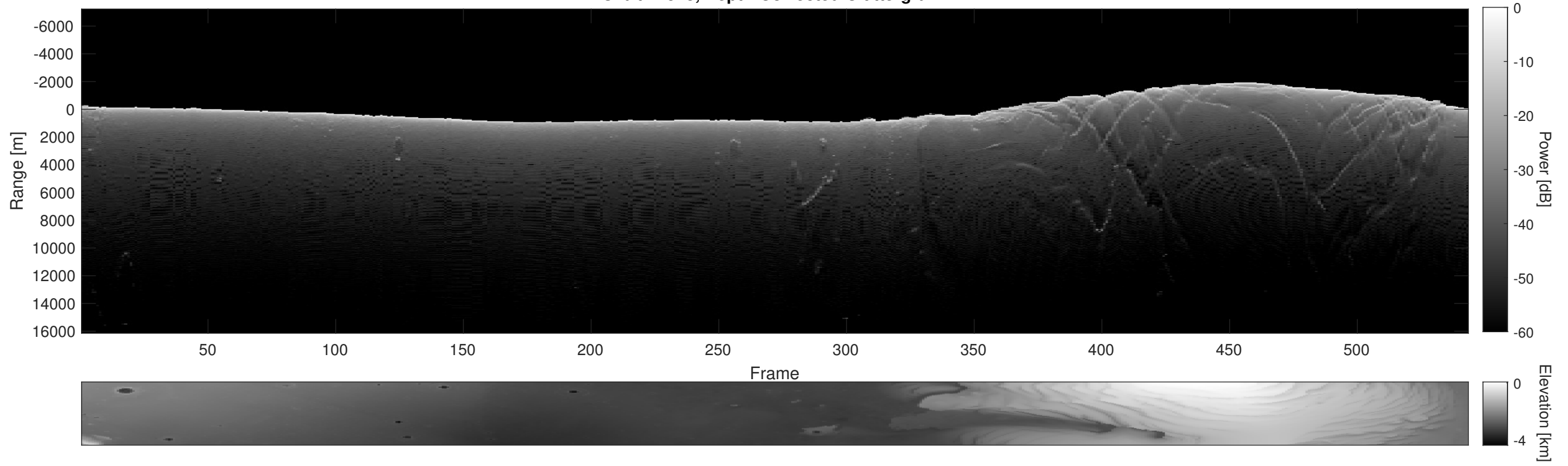
Orbit 22513, Depth-Corrected Cluttergram
