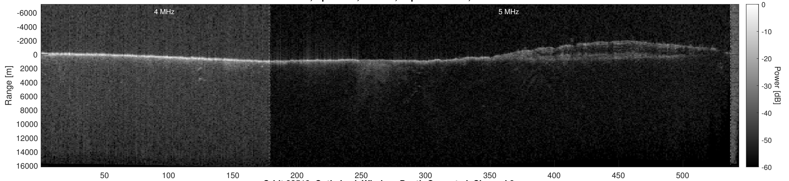
Orbit 22513, Optimized, Window, Depth-Corrected, Channel 2
