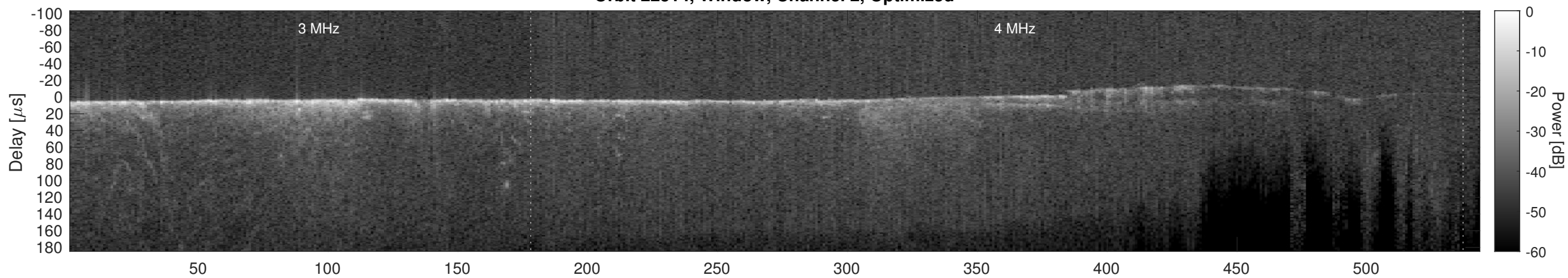
Orbit 22514, Cluttergram
