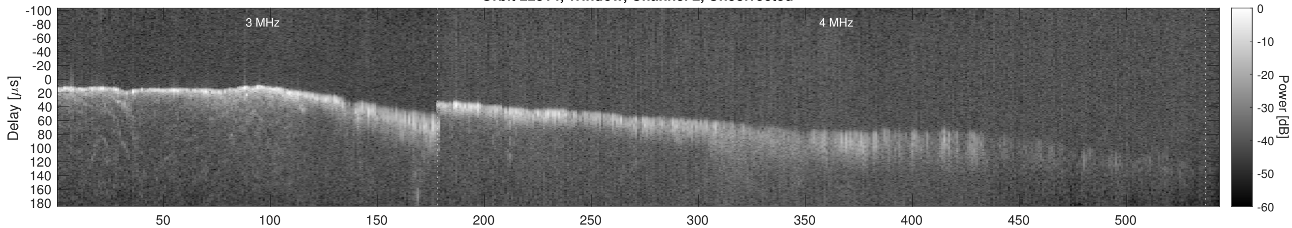
Orbit 22514, Window, Channel 2, Chapman
