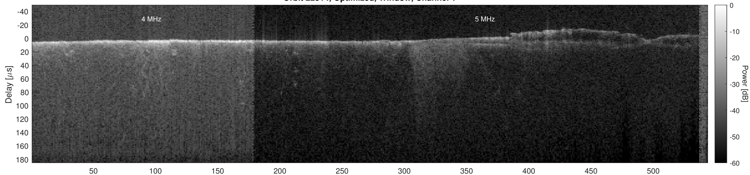
Orbit 22514, Optimized, Window, Channel 2
