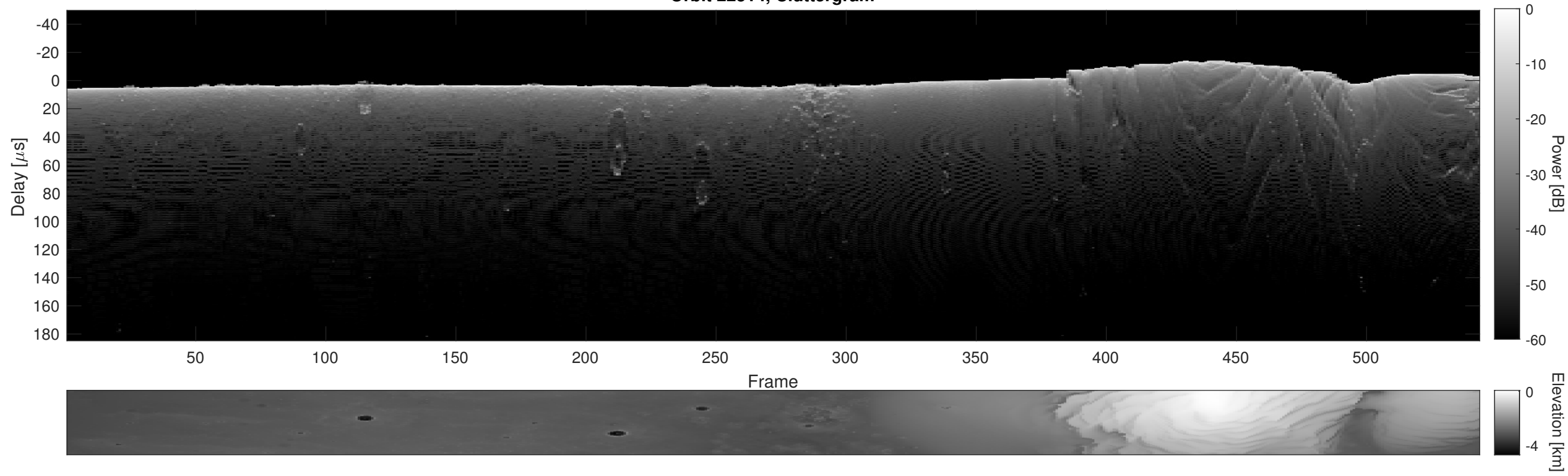
Orbit 22514, Cluttergram
