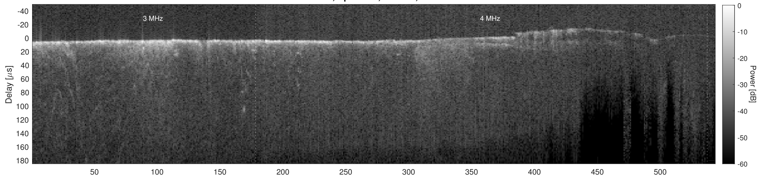
Orbit 22514, Cluttergram
